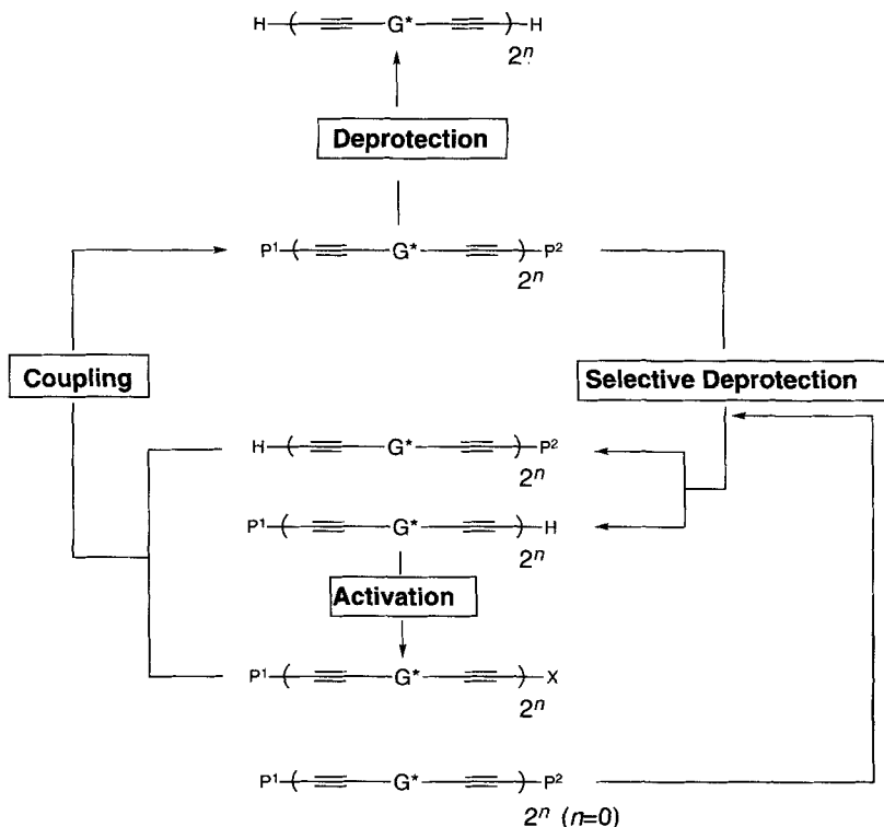
Scheme 1. Binomial Synthesis of Butadiyne-1,4-diyl-Linked Analogues of Oligo- and Polysaccharides *)
