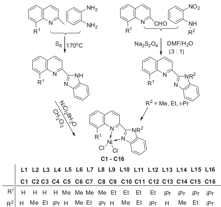
Scheme 1. Synthetic procedure.
