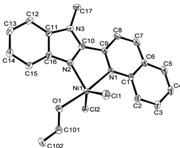
Figure 1. Molecular structure of C2 \cdot CH_3CH_2OH with thermal ellipsoids at the 30% probability level. Hydrogens have been omitted for clarity.
