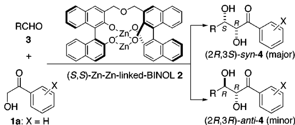
Scheme 1. syn -Selective Direct Catalytic Asymmetric Aldol Reaction Using (S,S)-Zn–Zn-Linked-BINOL Complex 2
