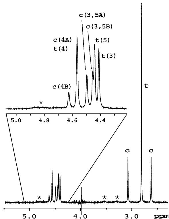
Figure 9. Cp region of the ^1\text{H} NMR spectrum of 3 in d_5 -pyridine at -50\text{ }^\circ\text{C} (20 mM). Labeling: c corresponds to cis - 5a ; t corresponds to trans - 5a ; * corresponds to a small amount of the mono-adduct 4a .
