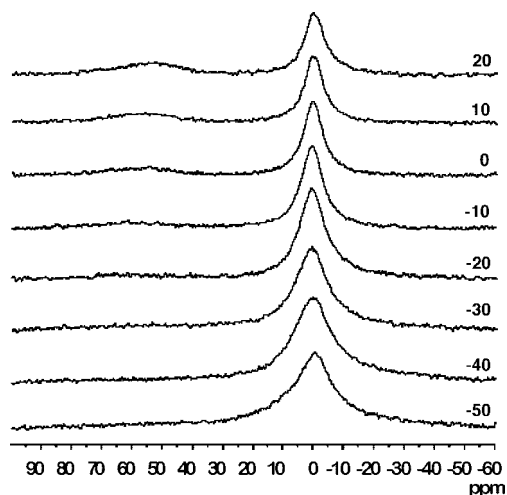
Figure 8. VT ^{11}\text{B} NMR spectra of 4a/5a in d_5 -pyridine (20 mM).
