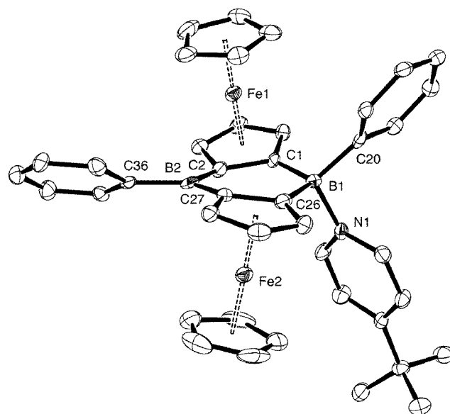
Figure 3. Molecular structure of 4b with thermal ellipsoids at the 50% probability level; hydrogen atoms are omitted for clarity. Fe1···B1 = 3.298; Fe1···B2 = 2.920, Fe2···B1 = 3.414; Fe2···B2 = 3.076 Å.
