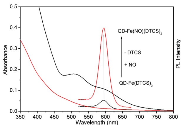
Figure 2. UV-vis absorption spectra of the \text{Fe(III)(DTCS)}_3 (black) before and (red) after the addition of nitric oxide. The photoluminescence spectra of the nanoprobe (black) before and (red) after the addition of nitric oxide. The PL intensities were normalized with respect to the absorbance.
