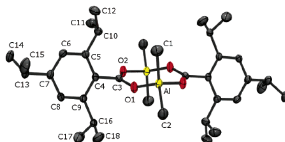
Figure 3. Molecular structure of [\text{Me}_2\text{Al}(\mu\text{-O}_2\text{CAr}^{\text{iPr}})]_2 ( 7 ), with atomic displacement parameters at the 50% probability level. Hydrogen atoms were omitted for clarity.
