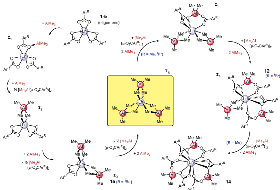
Scheme 7. Carboxylate–Alkyl Interchange: A Mechanistic Scenario of the Formation of Differently Alkylated Lanthanide Carboxylate Complexes a
