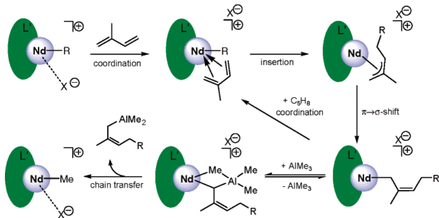
Scheme 9. Allyl Insertion Mechanism of 1,3-Diene Polymerization Taking into Account Organoaluminum-Mediated Chain Transfer
