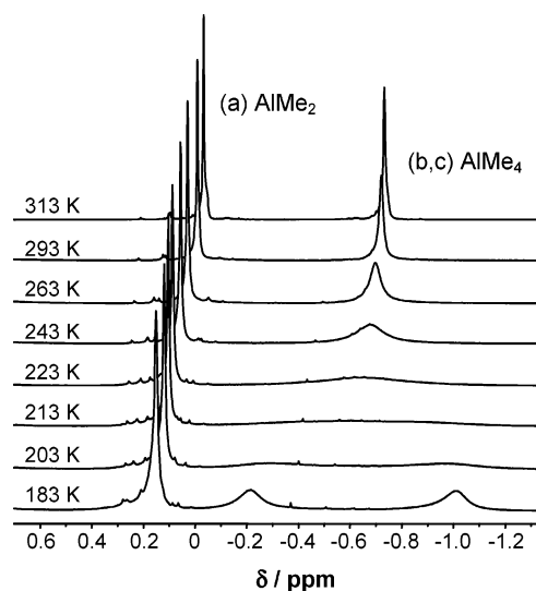
Figure 4. Region of the variable-temperature ^1\text{H} NMR spectra of 12b measured in toluene- d_8 (cf. Scheme 3).
