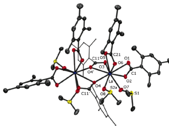
Figure 2. Molecular structure of [\text{La}(\text{O}_2\text{CC}_6\text{H}_2\text{Me}_3\text{-2,4,6})_2(\mu\text{-O}_2\text{CC}_6\text{H}_2\text{Me}_3\text{-2,4,6})(\text{DMSO})_2]_2 ( 1b' ), with atomic displacement parameters at the 50% probability level. The disorder over two positions at one of the two DMSO molecules (S2a, S2b) and all of the hydrogen atoms were omitted for clarity.
