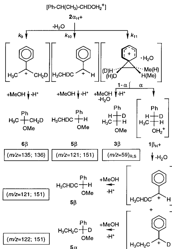
Scheme 5. Reaction pattern from gas-phase O-protonation of the diastereomeric mixture of 2-phenyl-1-deutero-1-propanol in the presence of methanol.
