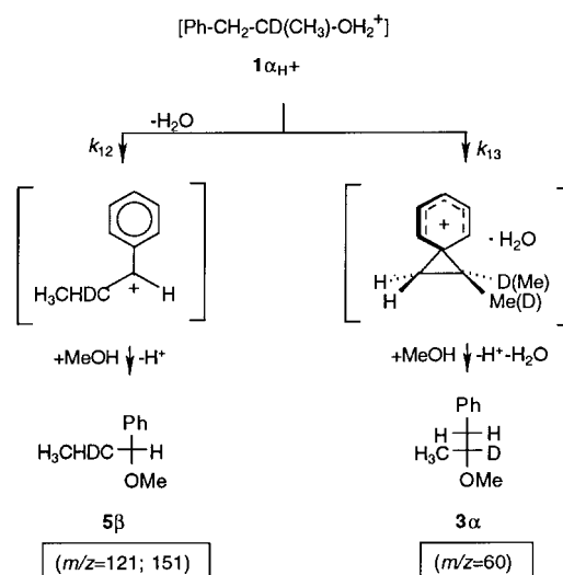
Scheme 6. Reaction pattern from gas-phase O-protonation of the racemate of 1-phenyl-2-deutero-2-propanol in the presence of methanol.
