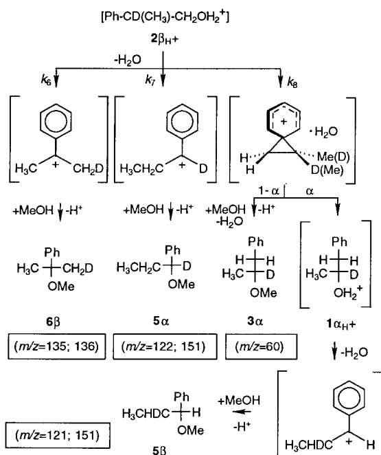
Scheme 4. Reaction pattern from gas-phase O-protonation of the racemate of 2-phenyl-1-deutero-1-propanol in the presence of methanol.
