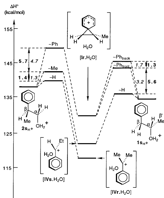
Figure 1. Energy profiles for adjacent group participations to \text{H}_2\text{O} loss in O-protonated (S)-1-phenyl-2-propanol ( 1s_{\text{H}^+} ) and O-protonated (S)-2-phenyl-1-propanol ( 2s_{\text{H}^+} ). The bold figures refer to the \Delta E^* and the italic ones to \Delta \log A^* (ref. [1]).
