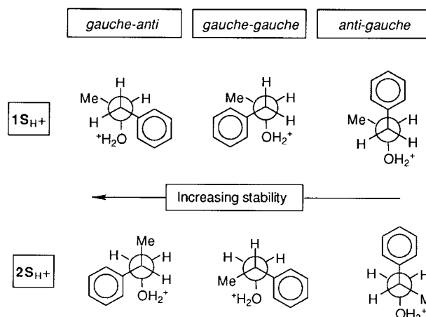
Scheme 1. Order of stability of the conformers of O-protonated (S)-1-phenyl-2-propanol and (S)-2-phenyl-1-propanol.
