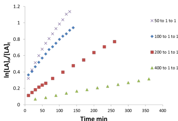
Figure 3: Kinetic plots at various [LA]:[Init]:[BnOH] ratios all at 80 °C, init = Al(1)Me 2 . Equations of lines of best-fit (50:1:1) y = 0.0067x + 0.31 ( R^2 = 0.986 ); (100:1:1) y = 0.0041x + 0.36 ( R^2 = 0.9867 ); (200:1:1) y = 0.0026x + 0.104 ( R^2 = 0.999 ); (400:1:1) y = 0.00075x + 0.04 ( R^2 = 0.998 ).
