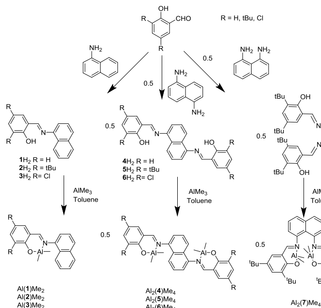
Figure 1: Preparation of the ligands and complexes used in this study.
