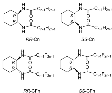
Chart 1 Molecular structures of RR-Cn , SS-Cn , RR-CFn or SS-CFn .
