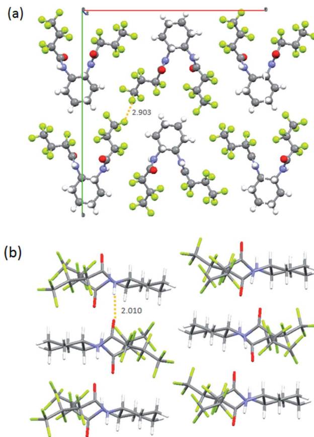
Fig. 5 The molecular structure and packing in a single crystal of racemic- CF4 .
