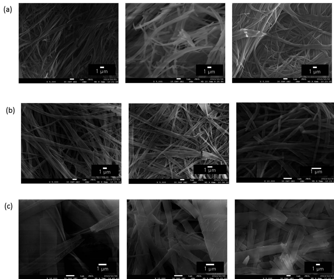
Fig. 2 The SEM images of the dried samples of C_6F_6 gels. Left; RR-CFn , middle; SS-CFn , right; racemic- CFn . (a) CF8 (b) CF9 (c) CF10.
