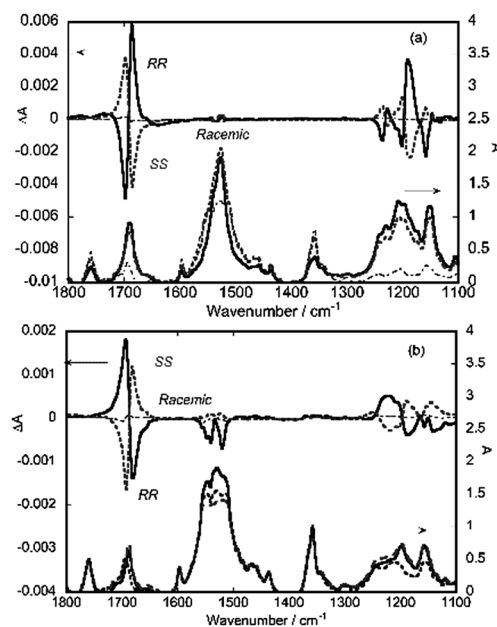
Fig. 3 The VCD (upper) and IR (lower) spectra of C_6F_6 gels containing enantiopure or racemic (a) CF8 ( 37.5\text{ g L}^{-1} ) and (b) CF9 ( 7.5\text{ g L}^{-1} ).
