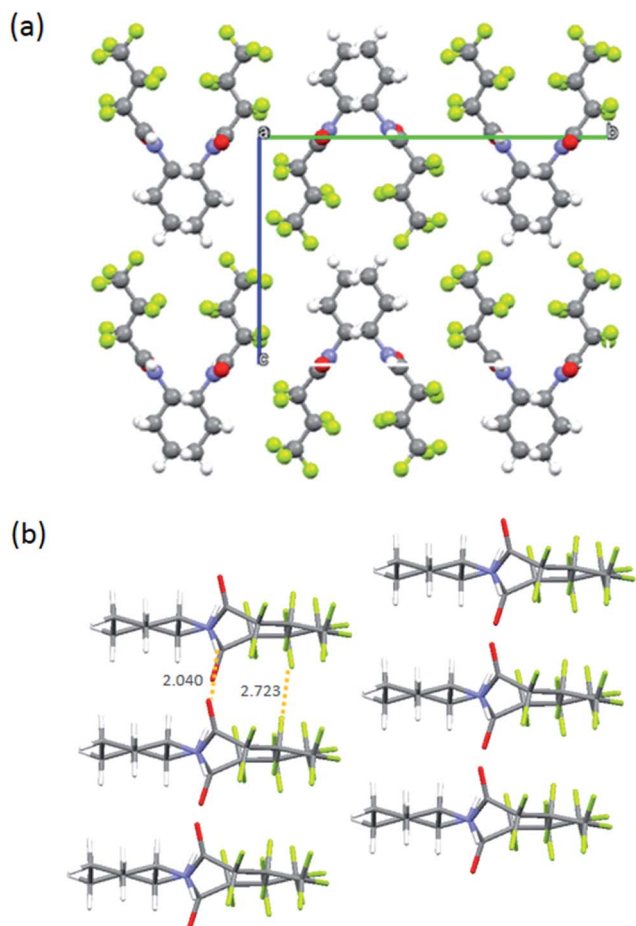
Fig. 4 The molecular structure and packing in a single crystal of RR-CF4 .
