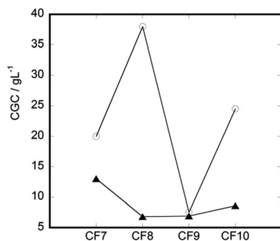
Fig. 1 The variation of the critical gel concentration of C 6 F 6 for racemic or enantiopure CF7–CF10. Open circle; chiral and solid triangle; racemic.
