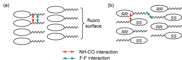
Fig. 6 The molecular models: (a) enantiopure-CFs, (b) racemic-CFs.
