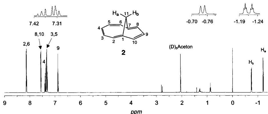
Fig. 3. ^1\text{H} -NMR Spectrum of homoazulene ( 2 ) (600 MHz; (\text{D}_6) acetone)
