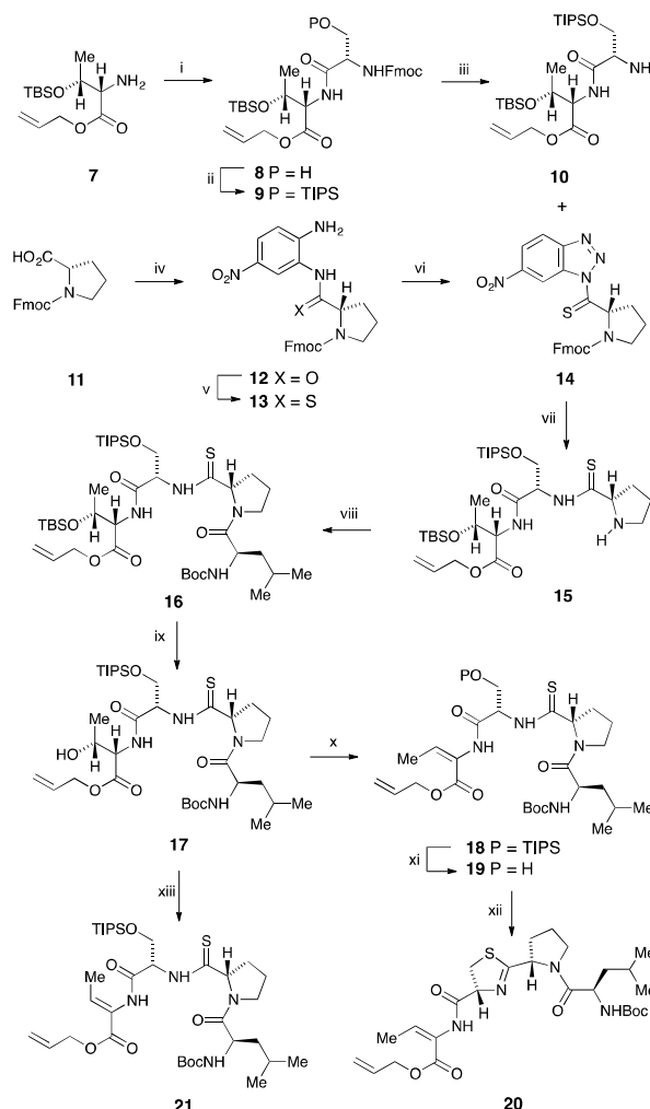
Scheme 2 Synthesis of the ( E )-dehydrobutyryne-thiazoline-L-pro-D-leu fragment 20 of vioprolide D Reagents and conditions i, Fmoc-L-ser, HATU, HOBT, \text{Pr}_2\text{NEt} , DMF, rt, 16 h (97%); ii, TIPSOTf, 2,6-lutidine (2,6-lut.), DCM, rt, 16 h (56%); iii, piperidine (pip.), DMF, rt, 16 h (89%); iv, 2-amino-4-nitroaniline, \text{tBuOC}(\text{O})\text{Cl} , N -methyl-morpholine (NMM), THF, -20^\circ\text{C} to rt, 16 h (79%); v, \text{P}_4\text{S}_{10} , \text{Na}_2\text{CO}_3 , THF, 0^\circ\text{C} , 30 min (71%); vi, \text{NaNO}_2 , glacial AcOH, \text{H}_2\text{O} , 0^\circ\text{C} , 30 min (86%); vii, (a) 10 , 14 , THF, rt, 6 h (66%) (b) pip., DMF, rt, 16 h (66%); viii, Boc-D-leu, HATU, HOBT, \text{Pr}_2\text{NEt} , DMF, rt, 16 h (85%); ix, (a) TBAF, THF, rt, 16 h (45%) (b) TIPSCl, imid., THF, rt, 48 h (68%); x, EDC, \text{CuCl}_2 (cat.), toluene, 80^\circ\text{C} , 30 min (65%); xi, TBAF, THF, rt, 16 h (62%); xii, DAST, -15^\circ\text{C} , 1 h (75%); xiii, DAST, py., 0^\circ\text{C} , 2 h (31%).
