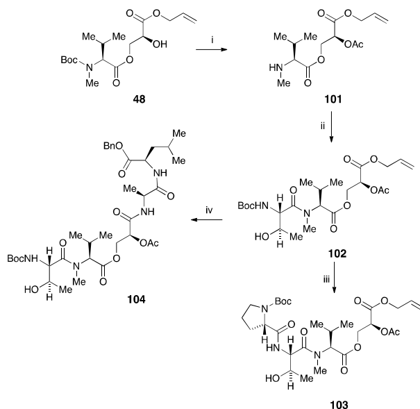
Scheme 14 Preliminary studies using the monoacetylated dipeptidyl glycerate 102 Reagents and conditions i, (a) Ac 2 O, DMAP, py., DCM, rt, 1.5 h (96%) (b) TFA, DCM, rt, 1.5 h (91%); ii, Boc-L-threonine, HATU, NMM, DMF, DCM, rt, 2.5 days (69%); iii, (a) 4N HCl, dioxane, 0 °C, 4 h (b) Boc-L-proline, i BuOC(O)Cl, NMM, THF, rt, 16 h (90%); iv, (a) Pd(Ph 3 P) 4 , PhSiH 3 , DCM, rt, 45 min (b) 60 , HATU, NMM, DCM, rt, 16 h (66%).
