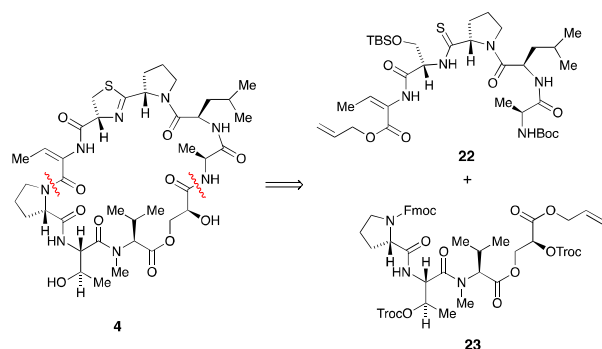
Figure 2 The convergent strategy conceived initially for a synthesis of vioprolide 4 .
