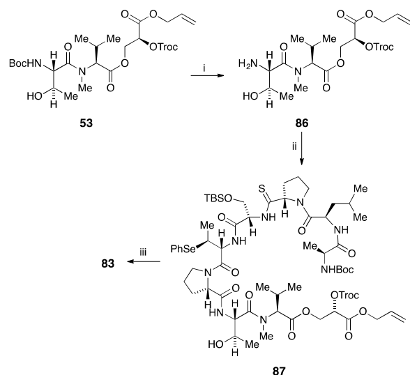
Scheme 10 An alternative synthesis of the octapeptidyl glyceride 83 Reagents and conditions i, 4N HCl, dioxane, 0 °C; ii, 81 , t BuOC(O)Cl, NMM, THF, -15 °C to rt, 17 h (79% from 53 ); iii, (a) activated Zn, AcOH, Et 2 O, rt, 16 h ( ca. 100%) (b) Ac 2 O, pyr., DMAP, DCM, 0 °C to rt (59%).
