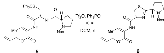
Scheme 1 Unsuccessful introduction of the thiazoline in the presence of an ( E )-dehydrobutyryne
