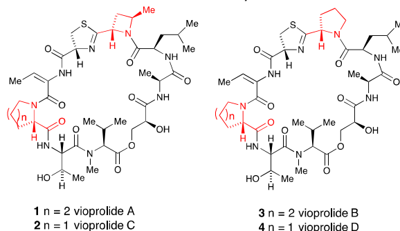
Figure 1 The structures of the naturally occurring vioprolides.
