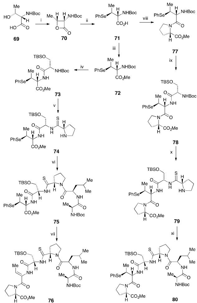
Scheme 8 Synthesis of the modified hexapeptide 80 Reagents and conditions i, PyBOP, \text{Et}_3\text{N} , DCM, rt, 2 h (74%); ii, \text{PhSeH} , DMF, 80^\circ\text{C} , 2 h (83%); iii, \text{TMSCHN}_2 , tol. , MeOH, rt, 2 h ( ca. 100%); iv, (a) TFA, DCM, rt, 2 h (b) HATU, HOBT, THF, O -TBS- N -Boc-L-ser., rt, 16 h (77%); v, (a) TFA, DCM, rt, 2 h (b) 14 , \text{Et}_3\text{N} , THF, rt, 16 h (c) pip. , THF, rt, 4 h (35% from 73 ); vi, 34 , HATU, HOBT, DCM, rt, 16 h (85%); vii, (a) NaOH, EtOH, dioxane, rt, 5 h (b) methyl L-prolinate, PyBOP, NMM, DCM, rt, 4.5 h (34%); viii, methyl L-prolinate, PyBOP, NMM, DCM, rt, 4 h (72%); ix, (a) TFA, DCM, rt, 1.5 h (b) O -TBS- N -Boc-L-ser., HATU, ^i\text{Pr}_2\text{NEt} , DCM, rt, 32 h (67%); x, (a) \text{TMSOTf} , 2,6-lut., DCM, rt, 2 h (b) 14 , ^i\text{Pr}_2\text{NEt} , DCM, rt, 16 h (66% from 78 ) (c) pip. , DMF, rt, 10 min (77%); xi, 34 , PyBOP, NMM, DCM, rt, 16 h (61%).
