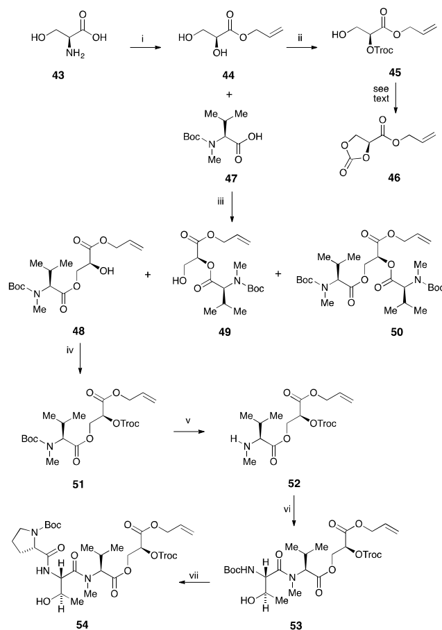
Scheme 5 Synthesis of the glyceric acid containing fragment 54 . Reagents and conditions i, (a) \text{NaNO}_2 , \text{HCl} , \text{H}_2\text{O} , 0^\circ\text{C} to rt, 24 h (71%); ii, (a) \text{TBSCl} , \text{DMAP} , \text{Et}_3\text{N} , \text{DCM} , rt, 17 h (56%) (b) \text{TrocCl} , \text{DMAP} , \text{py.} , \text{DCM} , rt, 17 h (66%) (c) \text{CuCl}_2 , acetone, \text{H}_2\text{O} , 57^\circ\text{C} , 16 h (87%); iii, \text{DCC} , \text{DMAP} , \text{DCM} , 0^\circ\text{C} to rt, 4 h ( 48 , 62%; 49 , 22%; 50 , 10%); iv, \text{TrocCl} , \text{DMAP} , \text{py.} , \text{DCM} , 0^\circ\text{C} , 3 h (97%); v, \text{TFA} , \text{DCM} , rt, 1 h (90%); vi, \text{Boc-L-threonine} , \text{DMF} , \text{DCM} , \text{HATU} , \text{NMM} , rt, 3.5 d (85%); vii, (a) 4\text{N HCl} , \text{dioxane} , 0^\circ\text{C} , 4 h (85%) (b) \text{Boc-L-proline} , \text{NMM} , \text{BuOC(O)Cl} , \text{THF} , rt, 15 h (77%).
