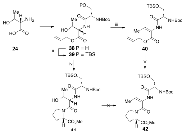
Scheme 4 Synthesis of the ( E )-dehydrobutyryne 40 Reagents and conditions i, (a) allyl alcohol, TsOH, toluene, 110 °C, 16 h (b) Boc-L-serine, HATU, HOBT, THF, 0 °C to rt, 16 h; ii, TBSCl, imidazole, THF, 0 °C to rt, 16 h (72% from 24 ); iii, EDC, \text{CuCl}_2 (cat.), toluene, 80 °C, 30 min (82%); iv, (a) \text{Pd}(\text{PPh}_3)_4 , \text{PhSiH}_3 , DCM, rt, 1 h (b) methyl L-prolinate, HOBT, PyBOP, NMM, DCM, rt, 16 h (42%).
