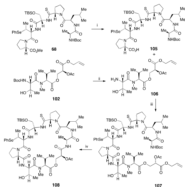
Scheme 15 Synthesis of the macrocycle 108 Reagents and conditions i, LiOH, t BuOH, THF, rt, 2 h (85%); ii, 4N HCl, dioxane, 0 °C, 4 h; iii, 105 , t BuOC(O)Cl, NMM, THF, -15 °C, 30 min, add 106 , THF, rt, 16 h (62%); iv, (a) Pd(Ph 3 P) 4 , PhSiH 3 , DCM, rt, 2 h (b) TFA, DCM, rt, 1 h (88% from 107 ) (c) HATU, HOBT, NMM, DCM, rt, 2.5 d (23%).
