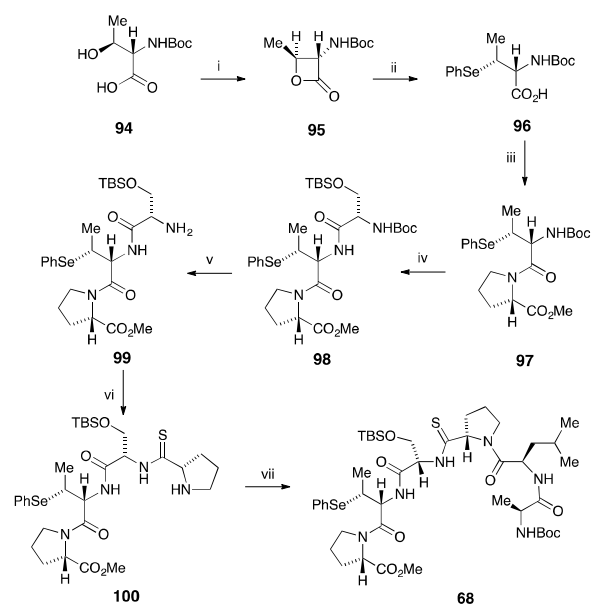
Scheme 13 Synthesis of the hexapeptide 68 Reagents and conditions i, PyBOP, Et 3 N, DCM, 0 °C, 1 h, rt, 1 h (95%); ii, PhSeH, DMF, 80 °C, 3 h (93%); iii, methyl L-prolinate, PyBOP, NMM, DCM, rt, 19 h (98%); iv, (a) TFA, DCM, 0 °C, 30 min (b) O -TBS- N -Boc-L-ser., HATU, i Pr 2 NEt, DCM, rt, 16 h (71%); v, TMSOTf, 2,6-lut., DCM, rt, 3 h (73%); vi, (a) 14 , i Pr 2 NEt, DCM, rt, 16 h (93%) (b) pip., DMF, rt, 15 min (83%); vii, 34 , PyBOP, NMM, DCM, rt, 17 h (93%).
