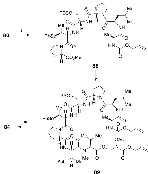
Scheme 11 An alternative synthesis of the macrocycle 84 Reagents and conditions i, (a) TMSOTf, 2,6-lut., DCM, rt, 1.5 h (b) CH 2 =CHCH 2 OC(O)Cl, Pr_2 NET, DMAP, rt, 16 h (58% from 80 ); ii, (a) LiOH, t BuOH, THF, 0 °C to rt, 2 h (b) 82 , t BuOC(O)Cl, NMM, THF, -20 °C to rt, 14 h (49%); iii, (a) Pd(Ph 3 P) 4 , PhSiH 3 , DCM, rt 1 h (b) PyBOP, NMM, DCM, 0 °C to rt, 64 h ( 84 , 33%).
