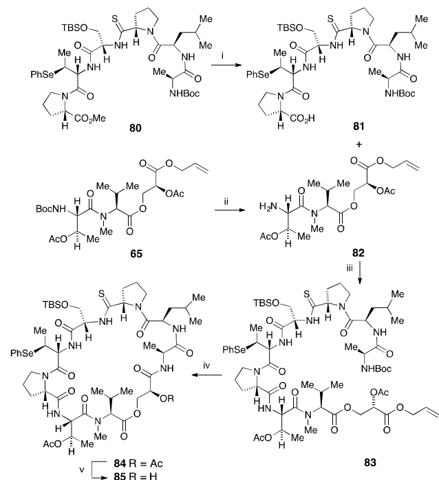
Scheme 9 Synthesis of a macrocyclic precursor of a ( Z )-iso-vioprolide Reagents and conditions i, LiOH, ^i\text{BuOH} , THF, 0^\circ\text{C} to rt, 2 h; ii, 4N HCl, dioxane, 0^\circ\text{C} , 4 h; iii, ^i\text{BuOC(O)Cl} , NMM, THF, -15^\circ\text{C} to rt, 20 h (84% from 65 ); iv, (a) \text{Pd(PPh}_3)_4 , \text{PhSiH}_3 , DCM, -15^\circ\text{C} to rt, 20 h (84% from 83 ); (b) TFA, DCM, 0^\circ\text{C} , 1 h (c) PyBOP, NMM, DCM, rt, 3 d (50% from 83 ); v, \text{Me}_3\text{SnOH} , DCM, 70^\circ\text{C} , 1.5 h (40%).
