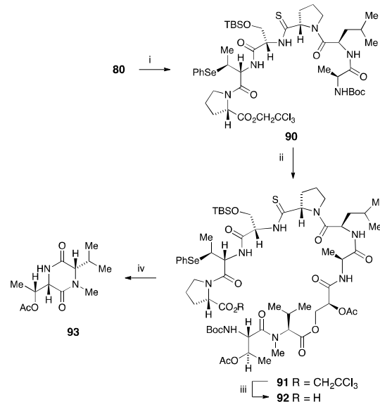
Scheme 12 Alternative assembly of the macrocycle from the two components Reagents and conditions i, (a) LiOH, t BuOH:THF (1:1), rt, 2 h (b) Cl 3 CCH 2 OH, EDC.HCl, DMAP, DCM, rt, 16 h (58%); ii, (a) TMSOTf, 2,6-lut., DCM, 2 h, rt (89%) (b) 66 , PyBOP, NMM, rt, 20 h (72%); iii, Zn, NH 4 OAc, THF, 0 °C to rt, 16 h; iv, HCl, dioxane, 4 h, 0 °C or TMSOTf, 2,6-lut., DCM.
