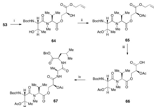
Scheme 7 Acetate protection of the glycerate Reagents and conditions i, activated Zn, AcOH, Et 2 O, rt, 2 h (96%); ii, Ac 2 O, DMAP, py., DCM, rt, 17 h (85%); iii, Pd(PPh 3 ) 4 , Ph 3 SiH, DCM, rt; iv, 60 , PyBOP, NMM, rt (85% from 65 ).
