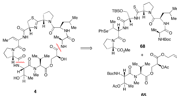
Figure 4 Revised strategy for a synthesis of vioprolide D 4
