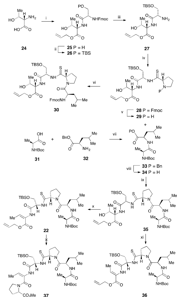
Scheme 3 Synthesis of the ( E )-dehydrobutyryne 22 Reagents and conditions i, (a) allyl alcohol, TsOH, toluene, 110 °C, 16 h (b) Fmoc-L-serine, HATU, HOBT, \text{Pr}_2\text{NEt} , 0 °C to rt, 16 h (74%); ii, TBSCl, imidazole, THF, rt, 16 h (79%); iii, pip., THF, rt, 3.5 h (68%); iv, 14 , THF, 0 °C to rt, 16 h (98%); v, pip., THF, rt, 4.75 h (95%); vi, Fmoc-D-leu, HATU, HOBT, rt, 16 h (75%); vii, \text{Et}_3\text{N} , DCM, EDC.HCl, HOBT, rt, 16 h (85%); viii, \text{H}_2 , Pd/C, EtOAc, rt, 16 h (96%); ix, HATU, HOBT, DCM, rt, 16 h (68%); x, EDC, \text{CuCl}_2 (cat.), toluene, 80 °C, 2.5 h (53%); xi, \text{Et}_3\text{N} , MsCl, DCM, 0 °C to rt, 30 min (58%).
