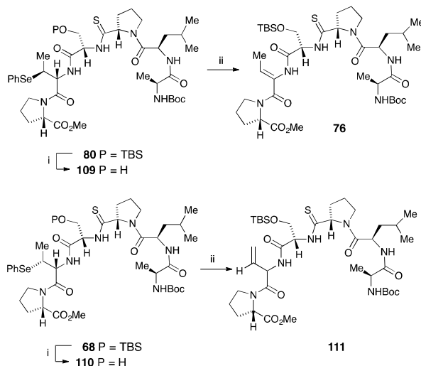
Scheme 16 Preliminary studies of oxidative elimination Reagents and conditions i, TBAF, THF, 0 °C, 5 min, rt, 2 h ( 109 , 92%; 110 , 92%); ii, t BuOOH, DCM, decane, 0 °C, 5 min, rt, 3 h ( 76 , 36%; 111 39%);
