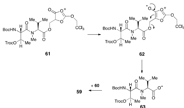
Figure 3 Possible explanation for loss of the glyceric acid moiety
