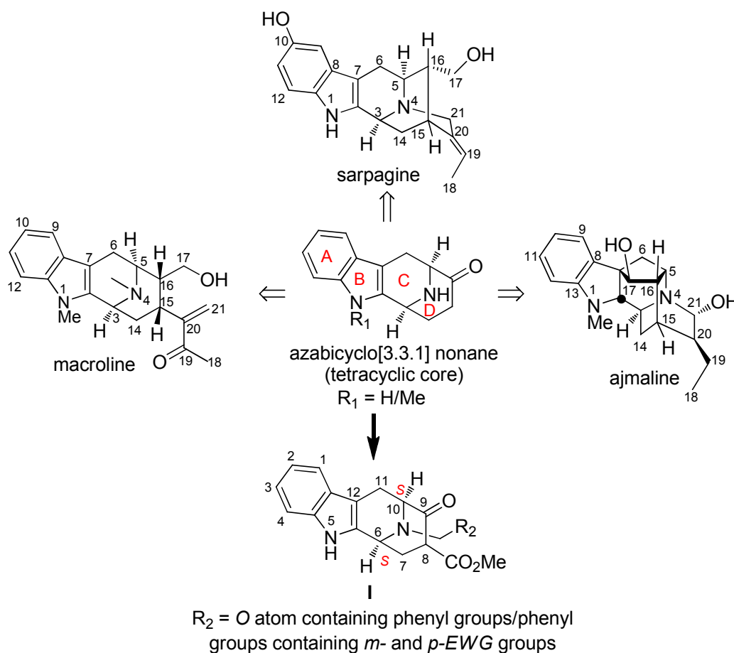
Figure 1. SAR of the cycloocta[ b ]indole framework (I) of the sarpagine - macroline and ajmaline related indole alkaloids active against MtpB. 7 EWG: electron withdrawing group.
