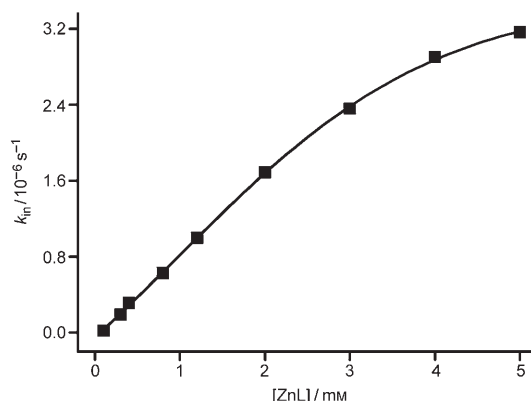
Figure 6. Dependence of the initial first-order rate constants on the concentration of ZnL at pH 8.85 and (308 \pm 0.1) \text{ K} ( I = 0.10 \text{ M} \text{NaClO}_4 , [\text{BNPP}] = 0.20 \text{ mM} , [\text{buffer}] = 50 \text{ mM} ).
