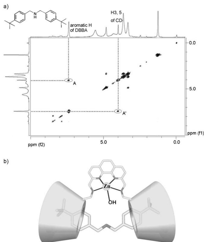
Figure 8. COSY spectrum of the inclusion complexation of ZnL and inhibitor DBBA.
