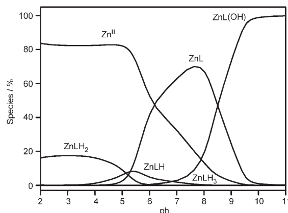
Figure 2. Distribution plots of species with ZnL (1.00 mM) as a function of pH at 0.10 \text{ M} \text{NaClO}_4 and (298 \pm 0.1) \text{ K} .
