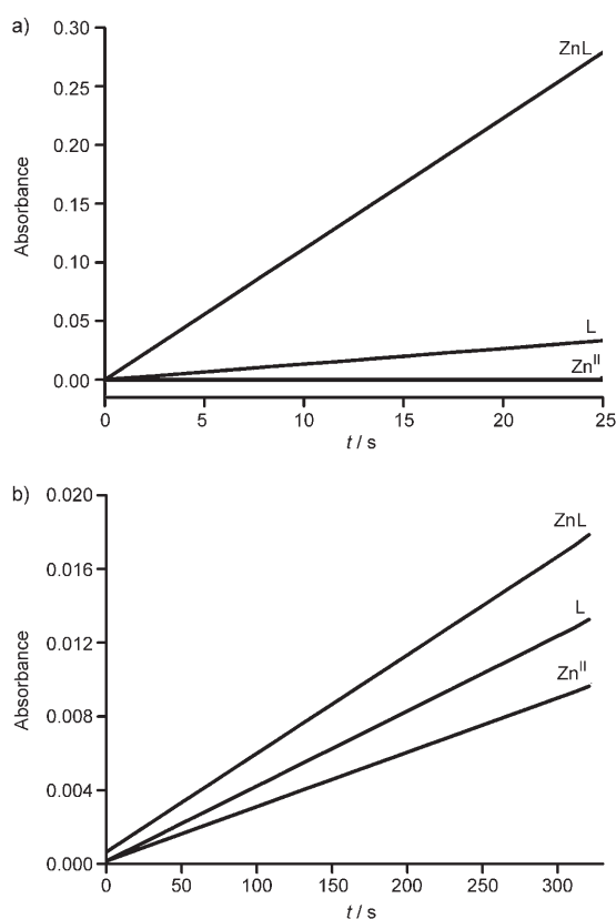
Figure 3. Plots of absorbance versus time during BNPC (a) and NA hydrolysis (b) catalyzed by \text{Zn}(\text{ClO}_4)_2 , L, and \text{ZnL} in a 10% MeCN solution of pH 7.01 Tris-HCl buffer with 0.10 M \text{NaClO}_4 at (298 \pm 0.1) K ([catalyst] = 50 \mu\text{M} , [BNPC] = 50 \mu\text{M} , [NA] = 200 \mu\text{M} ).
