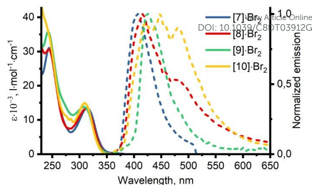
Fig. 6 Absorption at room temperature (solid lines) and phosphorescence emission (dashed lines) spectra of [7-10]·Br 2 in methanol/ethanol solution ( C = 20 \mu\text{M} ) at 80 K. Emission spectra were measured under excitation at \lambda_{\text{ex}} = 320 nm, delay 20 ns, gate 10 \mu\text{s} (30 \mu\text{s} for [8]·Br 2 ).
