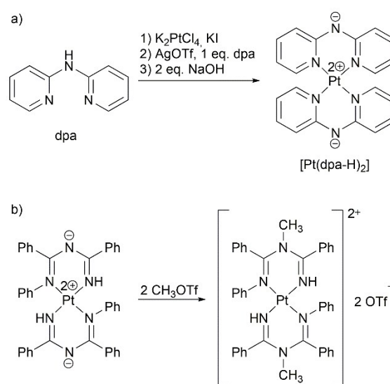
Scheme 3 Known reactions of platinum(II) complexes, which inspired this work: (a) synthesis of [Pt(dpa-H) 2 ] 23 (b) methylation of [Pt{NH=C(Ph)-NC(Ph)=NPh} 2 ] 26
