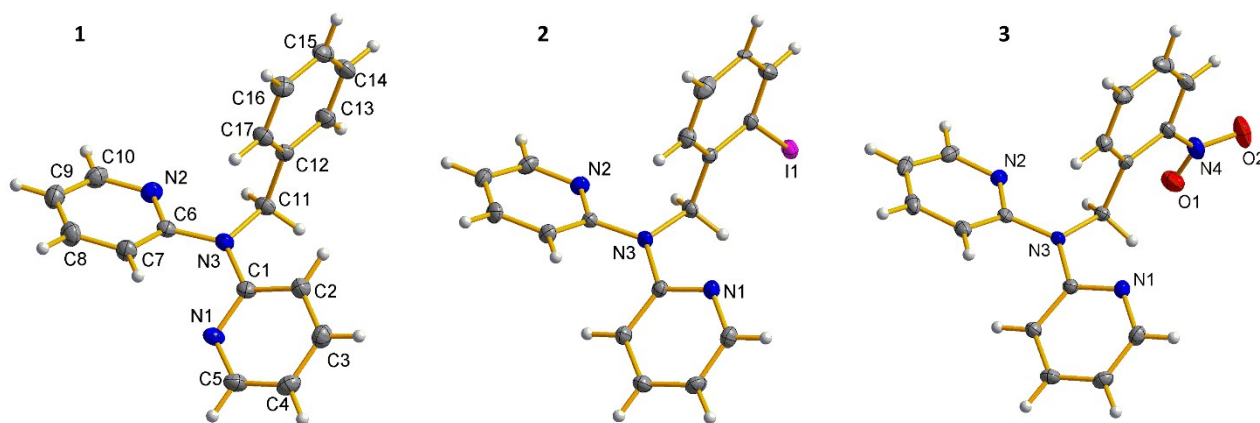
Fig. 1 Crystal structures of 1–3 .
