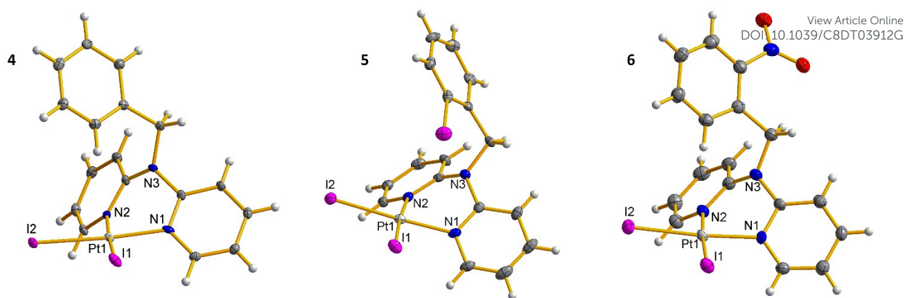
Fig. 3 Crystal structures of 4-6.
