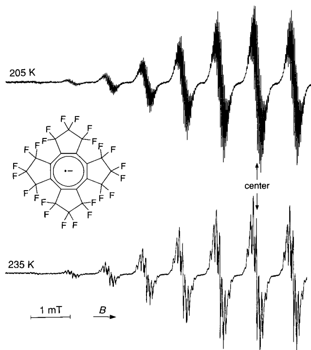
Fig. 4. Low-field parts of the ESR spectra of the radical anion 2 •- . Solvent: DME, counterion: K + , temperature as indicated.
