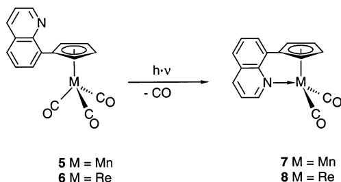
Scheme 4. Synthesis of 7 and 8 by photoinduced substitution of one CO ligand in 5 and 6 .
