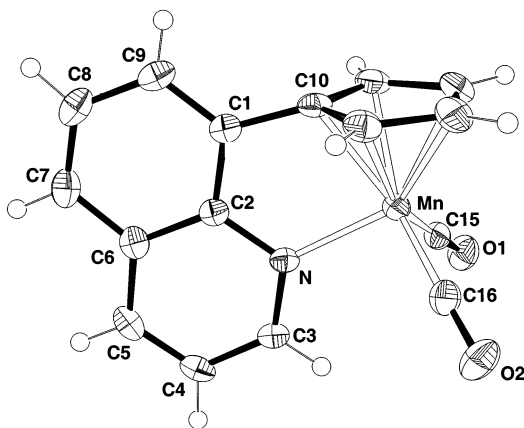
Fig. 3. Solid state structure of 7 , the structure of the Re complex 8 is very similar. Selected bond lengths (Å) and angles (°): (a) 7 , Mn–N 2.014(1); Mn–C Cp 2.12–2.14; Mn–C CO 1.78; C–O 1.16; C3–N–Mn 125.8(1); C2–N–C3 117.1(2); C2–N–Mn 117.0(1); C2–C1–C10 114.7(2); C9–C1–C10 126.2(2). (b) 8 , Re–N 2.123(3); Re–C Cp 2.26–2.30; Re–C CO 1.89–1.90; C–O 1.15–1.18; C3–N–Re 125.6(3); C2–N–C3 117.7(3); C2–N–Re 116.7(2); C2–C1–C10 117.5(3); C9–C1–C10 123.4(4).
