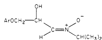
2 (Z isomer), Ar = 1-naphthyl
