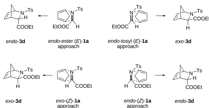
Scheme 3. Possible exo/endo - 3d transition pathways.
