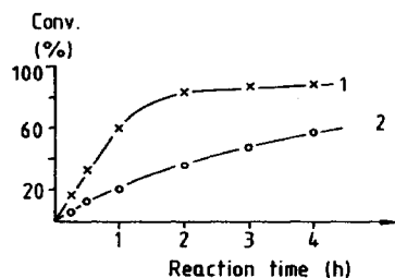
Fig. 1. Transfer hydrogenation of benzylideneacetophenone (1) and 1,5-cyclooctadiene (2). 2 \times 10^{-3} M catalyst; 1 mmol substrate in 12 ml 2-propanol; \text{NaOMe}:\text{Rh} = 10 ; 83^\circ\text{C} .
