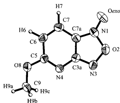
Figure 3. Crystallographic structure (ORTEP projection) of 5-methoxy-2-pyridofuroxan ( 7 )
