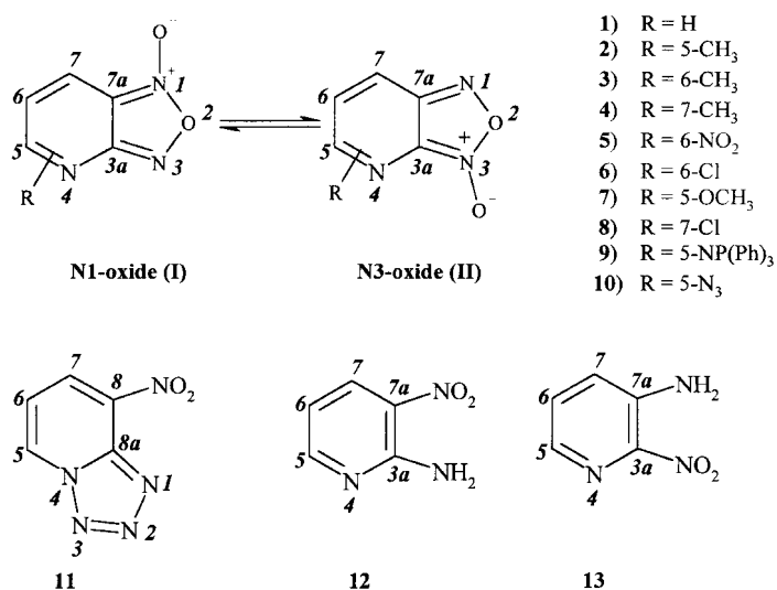
Figure 2. Numbering schemes and structures of the compounds studied. In the case of compounds 12 and 13 the numbering do not correspond to the IUPAC system
