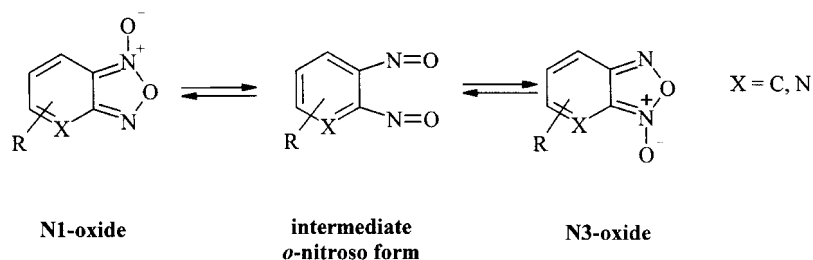
Figure 1. Valence tautomerism scheme for condensed furoxans
