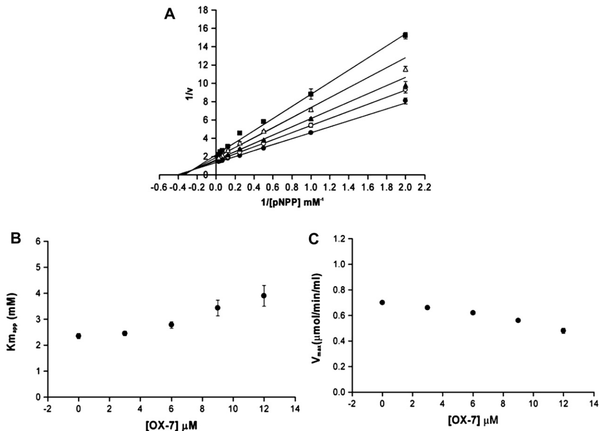
Fig. 8. [A] Compound OX-7 : double reciprocal plot ( 1/v versus 1/[S] ). The concentrations of inhibitor used were: 0 \mu\text{M} , \bullet ; 3 \mu\text{M} , \circ ; 6 \mu\text{M} , \blacktriangle ; 9 \mu\text{M} , \nabla ; 12 \mu\text{M} , \blacksquare . All tests were performed in quadruplicate. Dependence of main kinetic parameters K_m [B] and V_{\max} [C] from the concentration of compound OX-7 . The data represent the K_m or V_{\max} values \pm S.E.M.
