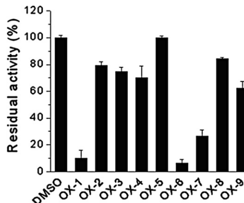
Fig. 2. Inhibition of PTP-1B activity by OX-1 – OX-9 compounds. Inhibition assays were performed at 37 °C and pH 7.0 at a fixed substrate final concentration (2.5 mM p -NPP), which is a value close to that of K m for PTP-1B at pH 7.0. The final concentration of each compound in the reaction assay was 40 μM. Each assay (final volume 1 ml) was started with 0.16 μg of PTP-1B. Control experiment was carried out using DMSO. Each datum represents the means ± S.E.M. of four distinct assays. Residual activity, expressed as percentage, is defined as the ratio between enzyme activity measured in the presence of the inhibitor and that of the control.
