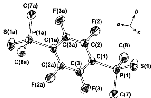
Figure 4. Molecular structure of 13 . Thermal ellipsoids are shown here at the 50% probability level. Hydrogen atoms have been omitted for clarity.
