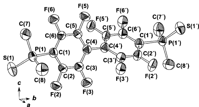
Figure 5. Molecular structure of 14 . Thermal ellipsoids are shown here at the 50% probability level. Hydrogen atoms have been omitted for clarity.
