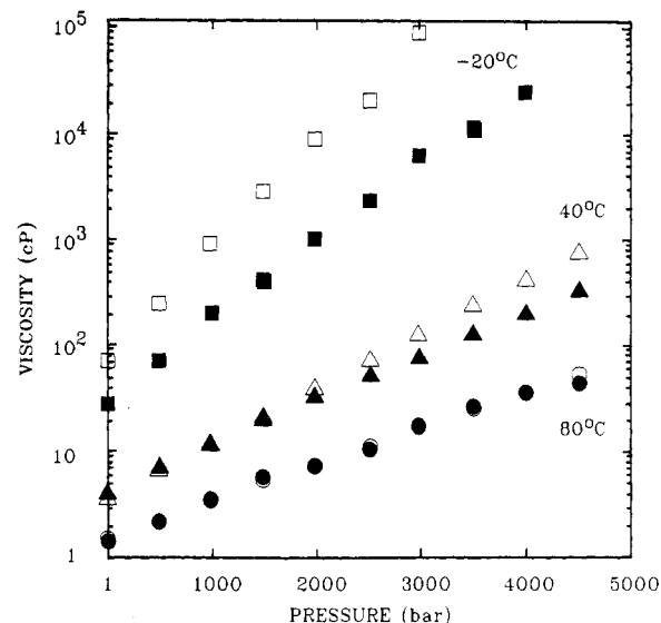
Figure 2. Pressure dependence of shear viscosity of EHC and EHB: □, EHB, -20 °C; △, EHB, 40 °C; ○, EHB, 80 °C; ■, EHC, -20 °C; ▲, EHC, 40 °C; ●, EHC, 80 °C.
