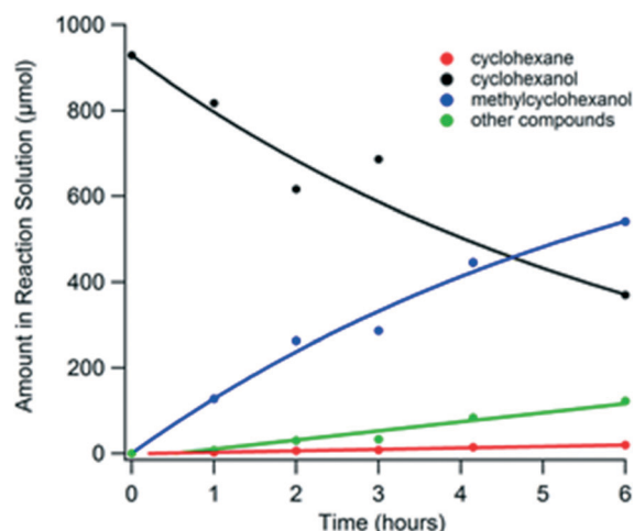
Fig. 5 Temporal evolution of products formed from cyclohexanol (ca. 1 mmol) in a batch reactor containing Cu20PMO in sc-MeOH ( T = 310\text{ }^{\circ}\text{C} ). Total material balance was greater than 99% after 6 hours.
