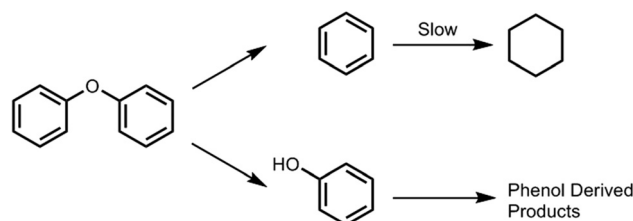
Scheme 3 Observed pathway for diphenyl ether (DPE).
