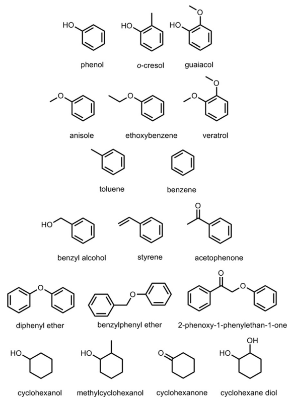
Fig. 2 Aromatic model compounds studied representing phenyl ether linkages and types of functional groups anticipated as intermediates in reductive lignin disassembly.
