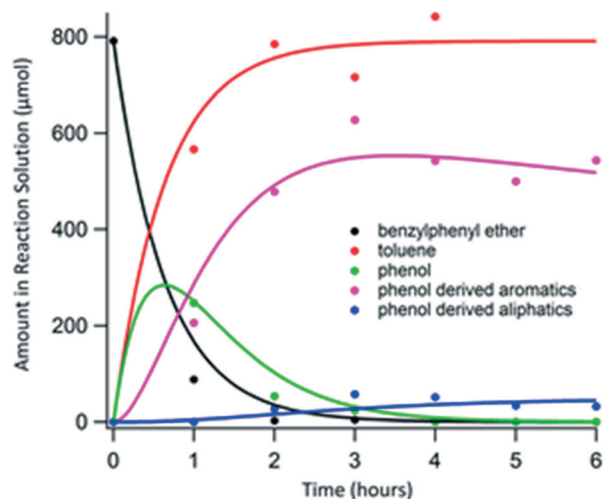
Fig. 6 Temporal product evolution for the reactions of benzyl phenyl ether in 2:1 MeOH:dimethyl-carbonate over Cu20PMO (300 °C). Material balance was 93% after 18 hours.
