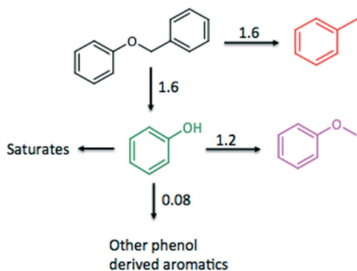
Scheme 7 Reactivity network for benzyl phenyl ether with Cu20PMO in 2:1 MeOH:DMC (300 °C).
