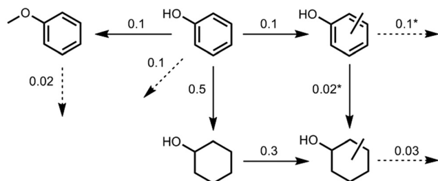
Scheme 1 Reaction network for phenol: (1 mmol substrate, 100 mg Cu 2 O/PMO, 3 mL MeOH, 310 °C). Observed rate constants are shown for each step, in units of h -1 . Dashed lines indicate conversion to unidentified compounds. Asterisks indicate rate constants fixed based on independent investigation of reaction products.
