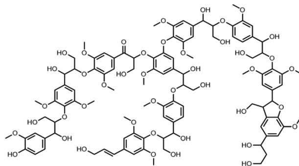
Fig. 1 A representative structure for a lignin fragment based on structural data by Sannigrahi et al. 7 and Stewart et al. 9
