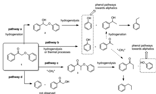
Scheme 5 Likely steps in disassembly of 2-phenoxy-1-phenylethane-1-one (1).
