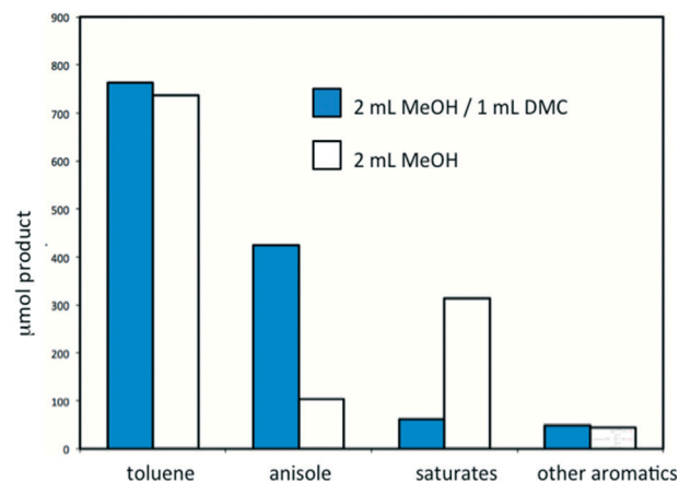
Fig. 7 Changes in product distribution upon using dimethyl carbonate as a cosolvent vs. using MeOH only. Products after 6 h reaction.
