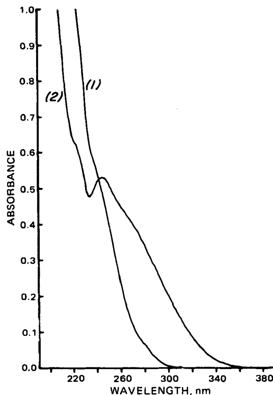
Figure 3—UV spectra of photoproduct (Z-isomer) in pH 4.4 buffer (1) and pH 10.8 buffer (2).
