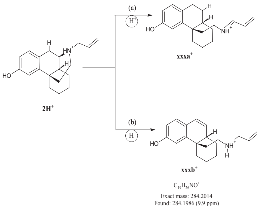
SCHEME 3. Formation of product ions xxxa^+ and xxxb^+ from 2H^+ .
