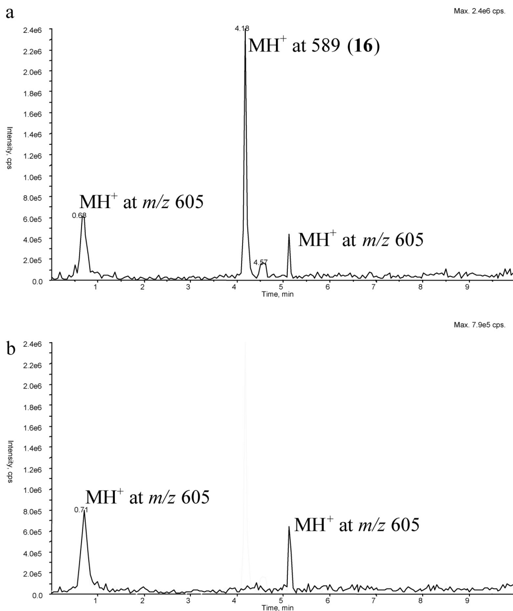
FIG. 6. TIC from the HPLC/MS experiment of the incubation mixture of levallorphan (10 \mu\text{M} ) supplemented with NADPH and GSH with recombinant CYP3A4 (a) and recombinant CYP2D6 (b).
