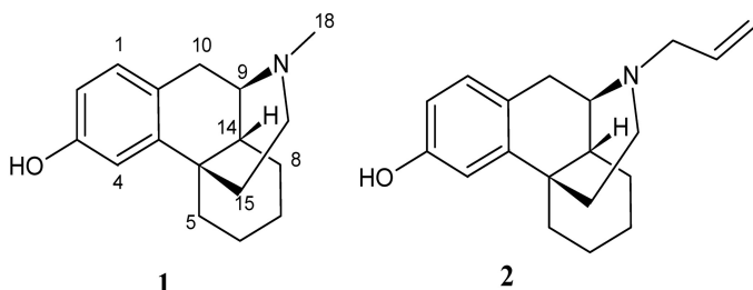
FIG. 1. Structures of levorphanol (1) and levallorphan (2).
