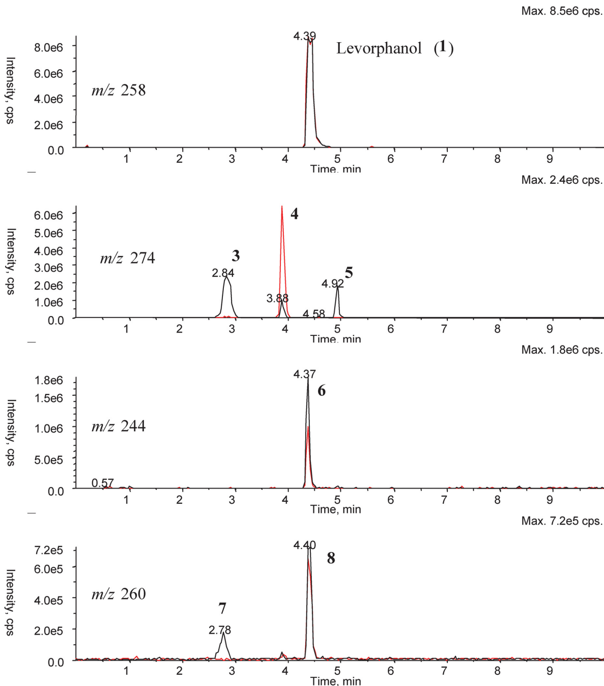
FIG. 3. XICs obtained from extracts of incubation mixtures of levorphanol (10 \mu M ) in the presence of NADPH-supplemented recombinant CYP3A4 (black) and CYP2D6 (red).
