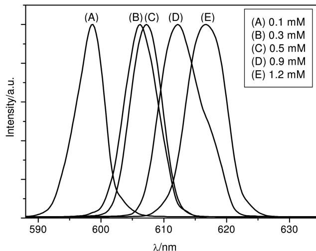
Figure 5. Lasing efficiencies in ethanol of PTalk (black bars) and PTAr (ray bars) (upper figure) and laser emission spectra of PTalk in ethanol as a function of the dye concentration.
