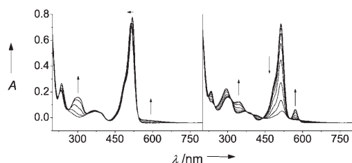
Figure 4. Spectroelectrochemistry of (pS-1)_2 . First reduction (left) and second reduction to the typical BDP radical dianion (right) in MeCN/0.2 M TBAH.
