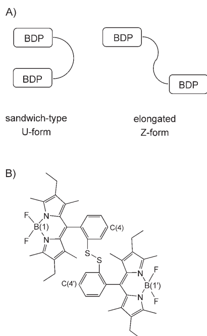
Scheme 3. A) Two possible conformers of (oS-1) 2 with maximum (U-form) and minimum (Z-form) chromophore–chromophore interaction. The apparent torsion angles between atoms B1-C4-C4'-B1' (see B) obtained for the two stable U- and Z-conformations of (oS-1) 2 by ground-state geometry optimization by the AM1 method are -61^\circ for the U-form and -134^\circ for the Z-form.
