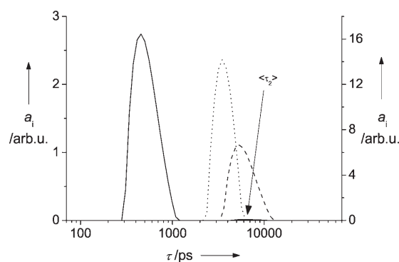
Figure 2. Representative lifetime distribution functions of (oS-1)_2 in DMSO (solid, minor mode indicated by the arrow) and THF (dashed), as well as (pS-1)_2 in MeCN (dotted), obtained for 494/564 nm excitation and emission wavelengths. For data, see Table 2.
