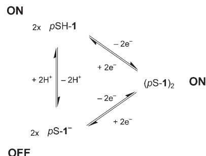
Scheme 2. Illustration of the switching states and processes of the title compounds.
