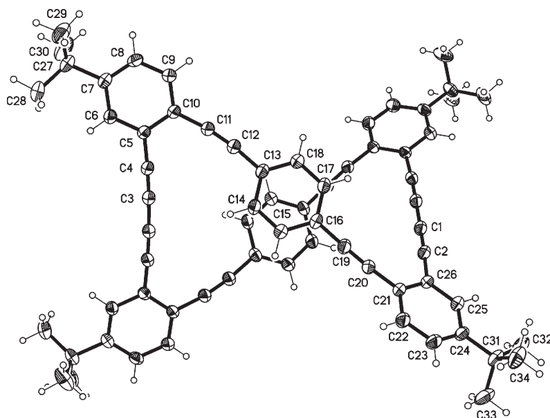
Figure 1. Molecular structure of 12b ; ellipsoids are drawn with 50% probability.
