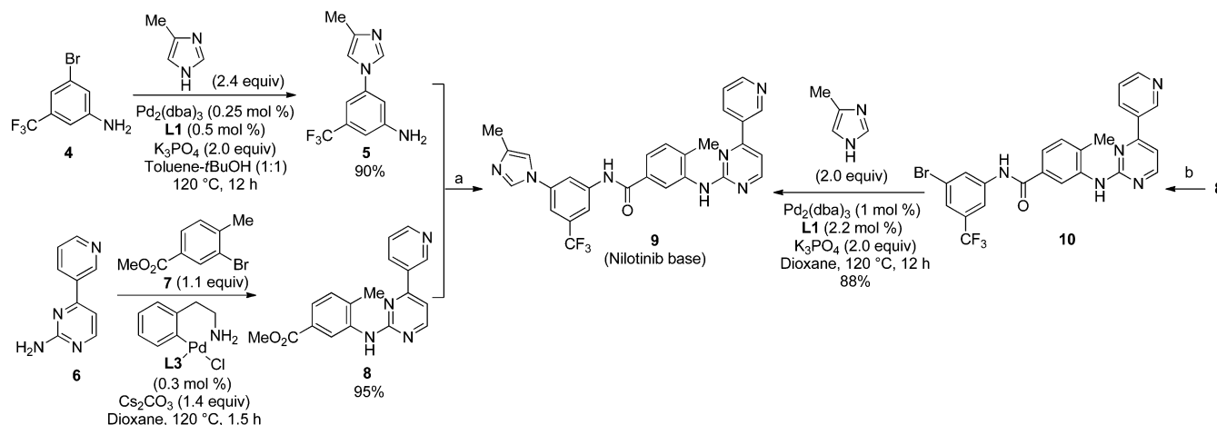
Scheme 4. Synthesis of Nilotinib Base a
