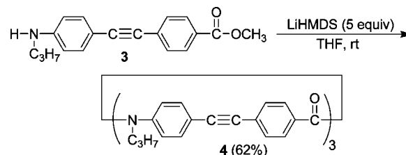
Scheme 2. Condensation of Diphenylacetylene Monomer 3
