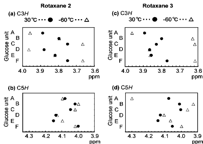
FIGURE 4. Results of the peak shifts of inner protons ( \text{C3H} and \text{C5H} ) of modified \alpha -CDs from 30 °C to –60 °C. (a and b) Protons of \text{C3H} and \text{C5H} in rotaxane 2, respectively. (c and d) Protons of \text{C3H} and \text{C5H} in rotaxane 3, respectively. A vertical scale (A–F) represents the glucopyranose unit.
