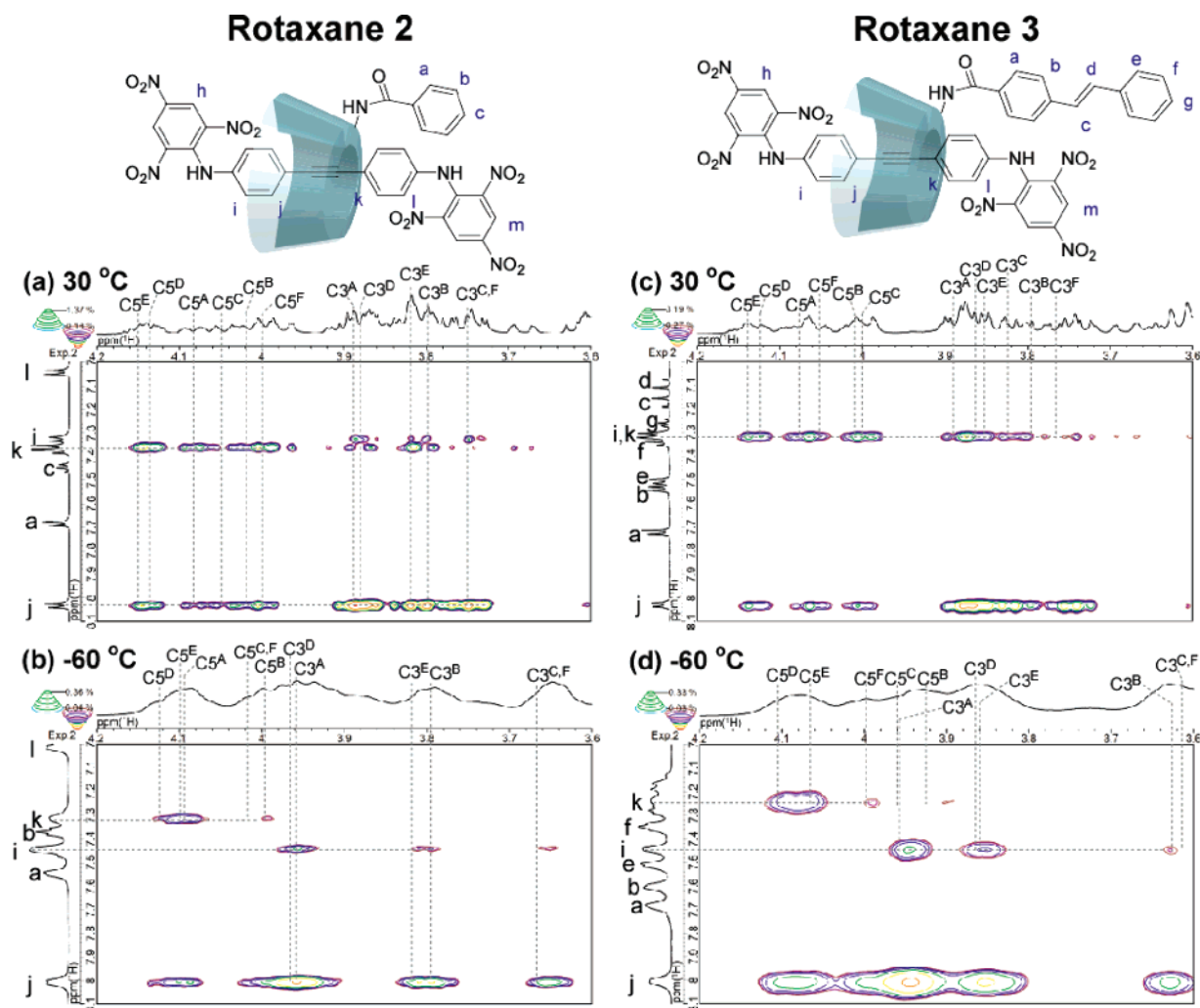
FIGURE 5. ROESY NMR spectra of rotaxanes 2 (a and b) and 3 (c and d) in methanol- d_4 (5 mM) under variable temperature.
