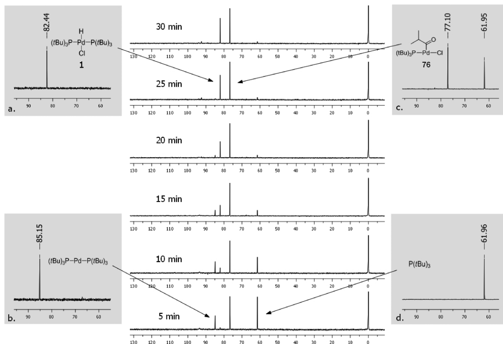
Figure 4. ^{31}\text{P} NMR spectra of the catalyst mixture in saffrole and its evolution over time.
