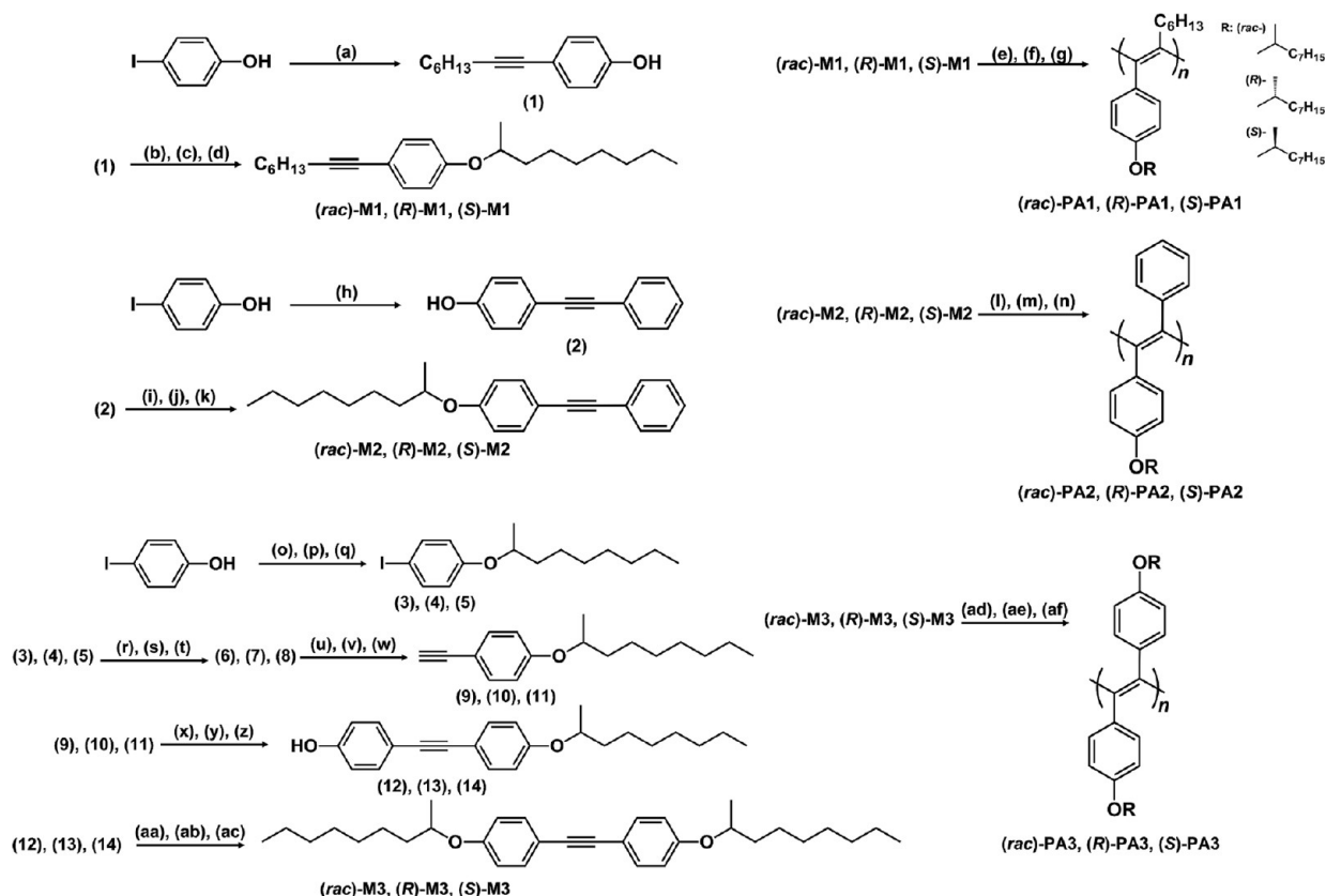
Scheme 2. Synthesis Routes for the Monomers and Disubstituted LCPC Derivatives a
