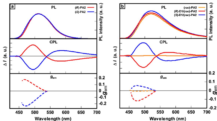
Figure 6. PL (upper), CPL spectra (middle), and g_{em} (lower) spectra of (a) (R)/(S)-PA2 N*-LC film, and (b) (R)/(S)-D1-doped (rac)-PA2 (10 wt%) N*-LC film. The measurements were performed with excitation using unpolarized light at 367 nm.
