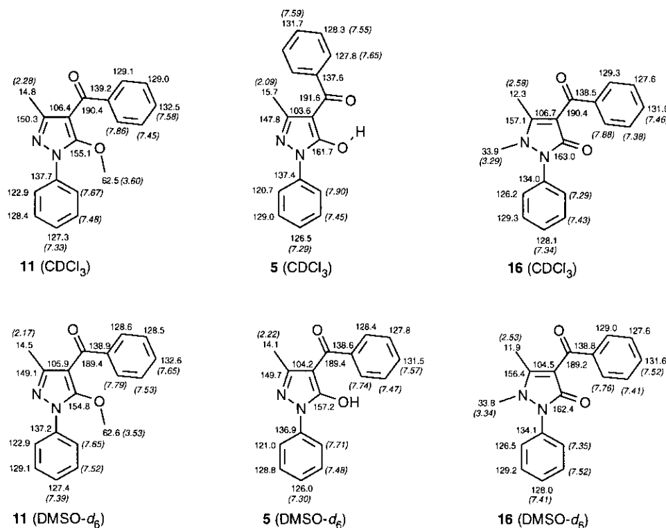
Figure 1. ^{13}\text{C} -NMR chemical shifts and ^1\text{H} -NMR chemical shifts (in italics) of pyrazolone ( 5 ) and its O -methyl ( 11 ) and N -methyl ( 16 ) congener in \text{CDCl}_3 and \text{DMSO}-d_6 solution.
