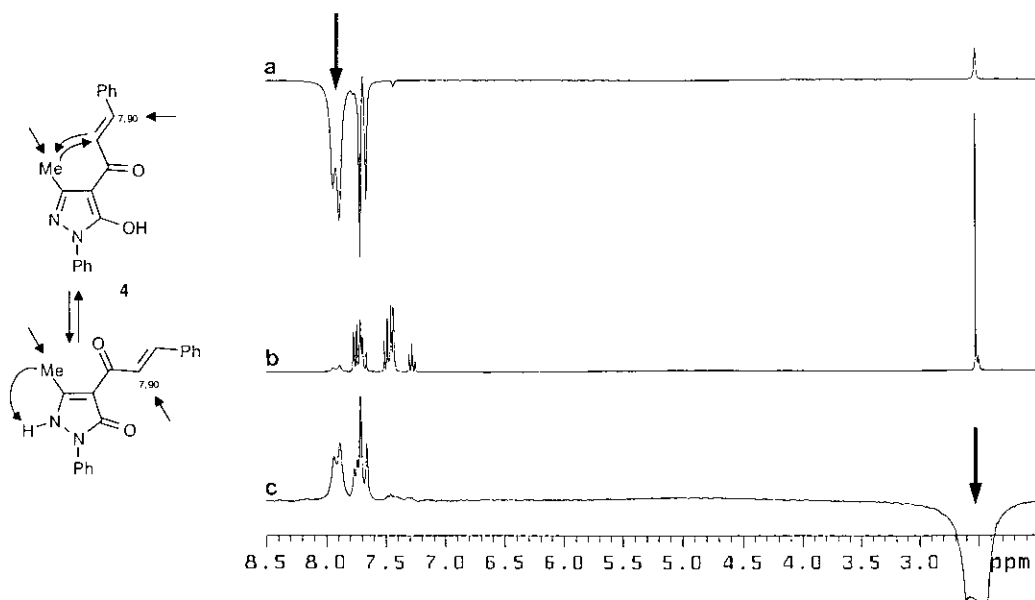
Figure 3. NOE-Difference experiments with 4 in DMSO- d_6 solution. a: NOE-difference spectrum obtained upon irradiation of d (1H) 7.90 ppm. b: ^1\text{H} -NMR spectrum of 4 . c: NOE-difference spectrum obtained upon irradiation of 3-Me.
