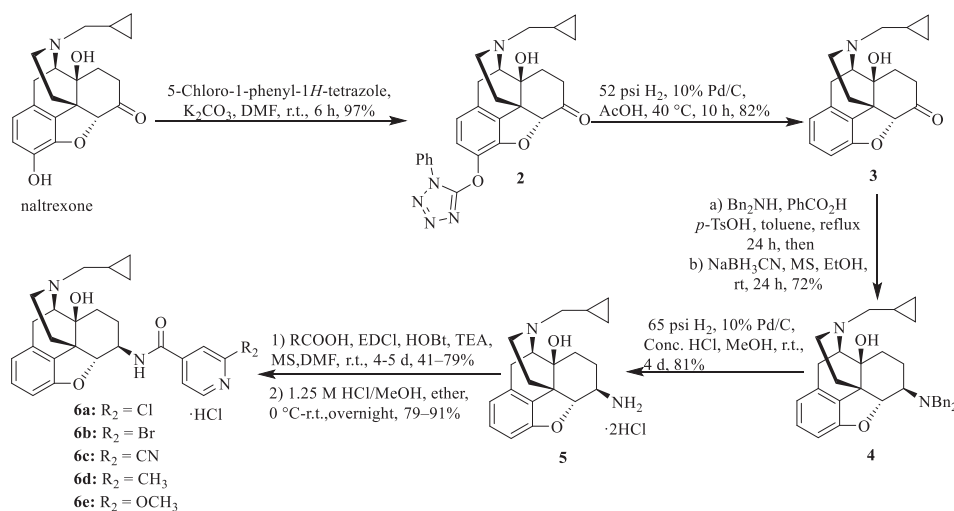
Scheme 1. Synthesis of the target compounds 6a-e .
