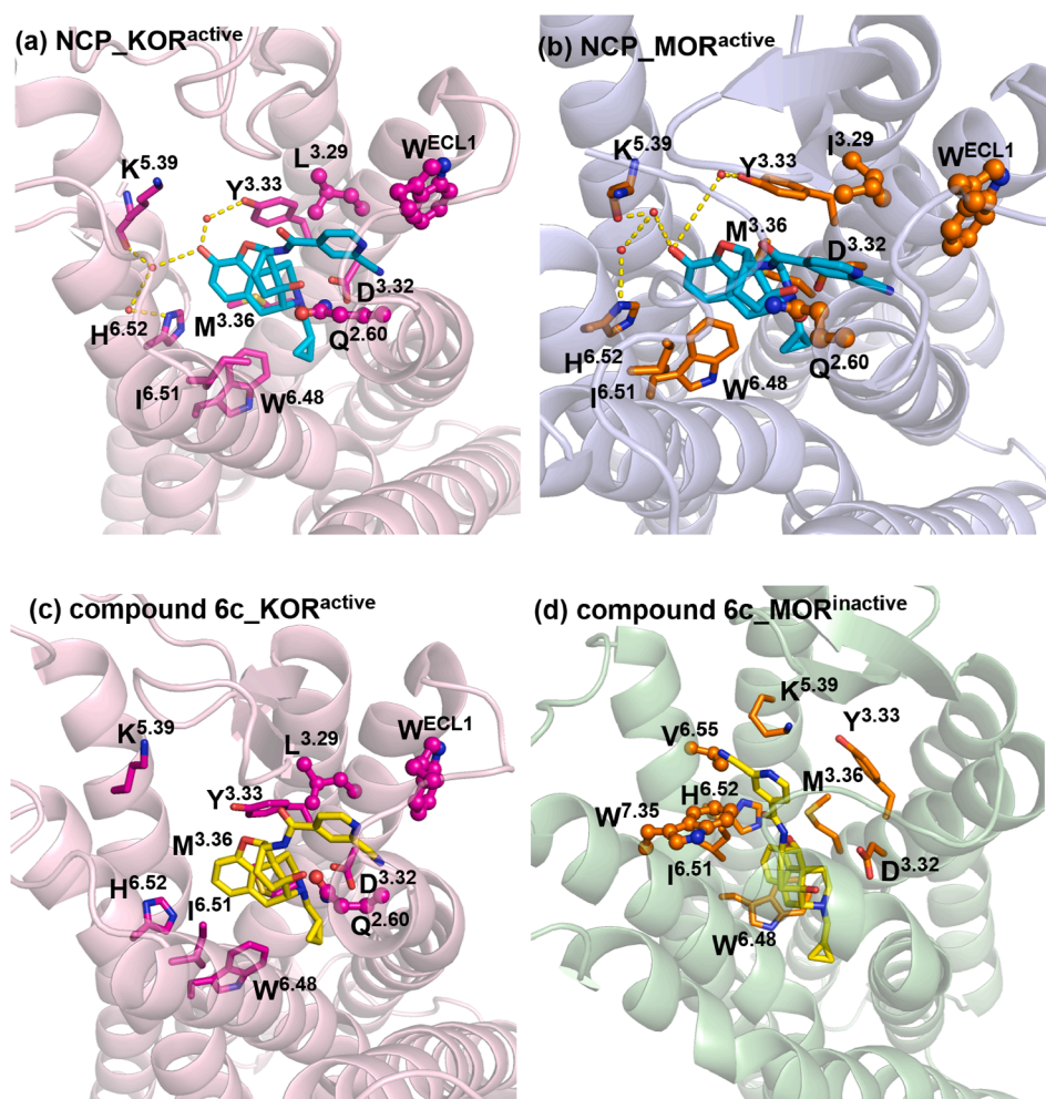
Fig. 6. The binding modes of \text{NCP}_{\text{KOR}}^{\text{active}} , \text{NCP}_{\text{MOR}}^{\text{active}} , compound 6\text{c}_{\text{KOR}}^{\text{active}} , and compound 6\text{c}_{\text{MOR}}^{\text{inactive}} complexes after 100 ns MD simulations. The receptors were shown as cartoon models, the active KOR in light-pink, the active MOR in light-blue, and the inactive MOR in light-green. NCP, compound 6c, and key amino acid residues were shown as stick models. Carbon atoms: NCP in cyan; compound 6c in yellow; key amino acid residues of the KOR in magenta, and the MOR in orange. The dashed lines in yellow represented potential water-mediated hydrogen bonds. The key residues at the allosteric site of the MOR were shown as stick and ball models in magentas. The key residues at the allosteric site of the KOR were shown as stick and ball models in orange. The water molecules were shown as sphere models in red. (For interpretation of the references to colour in this figure legend, the reader is referred to the web version of this article.)
