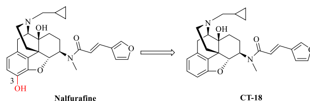
Fig. 3. Chemical structures of nalfurafine and compound CT-18 .
