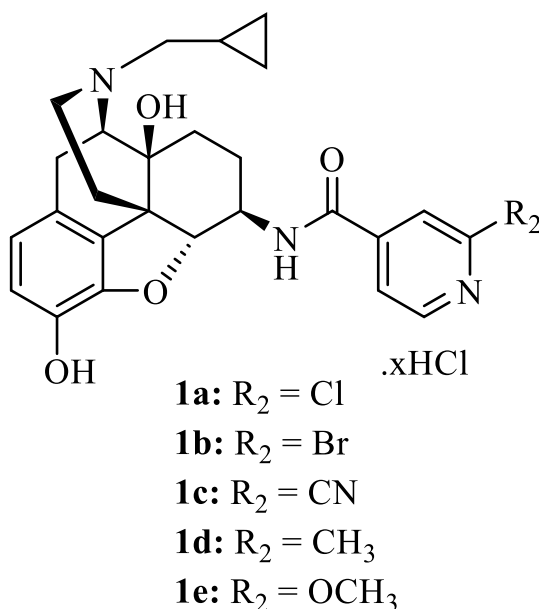
Fig. 1. Chemical structures of compounds 1a–e .
