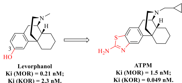
Fig. 4. Chemical structures of levorphanol and compound ATPM.
