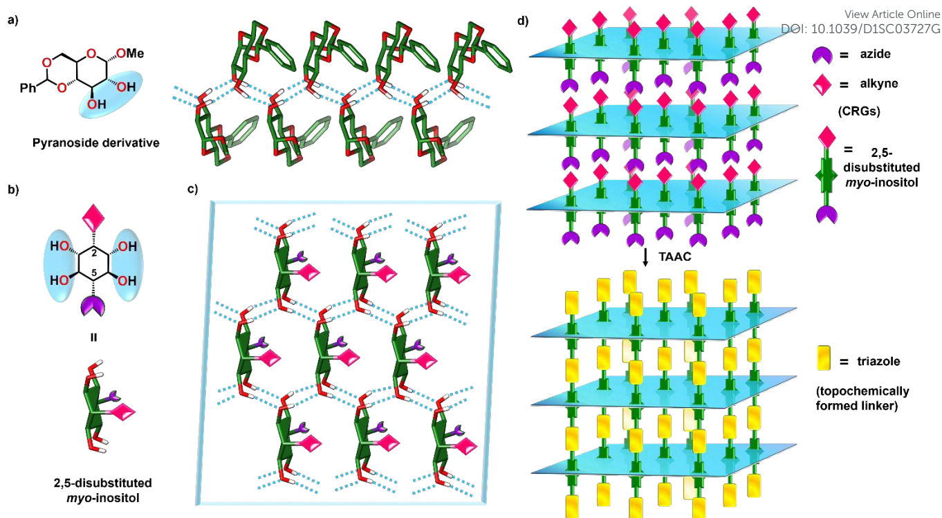
Fig. 2 a) 1D hydrogen-bonded zigzag arrangement in crystal structures of a representative pyranoside derivative possessing diequatorial vicinal diol. b) myo -inositol derivative decorated with CRGs at 2- and 5-positions. c) Expected 2D hydrogen-bonded layer in the myo -inositol derivative. d) Proposed head-to-tail arrangement of myo -inositol derivatives having CRGs at 2- & 5-positions and their topochemical polymerization reaction.
