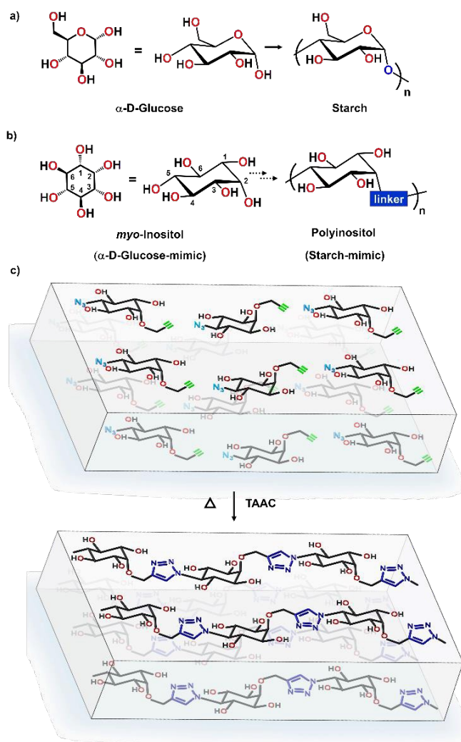
Fig. 1 a-b) Structural similarities of α-D-glucose and myo -inositol & starch and polyinositol. c) Schematic representation of SCSC synthesis of polyinositol.
