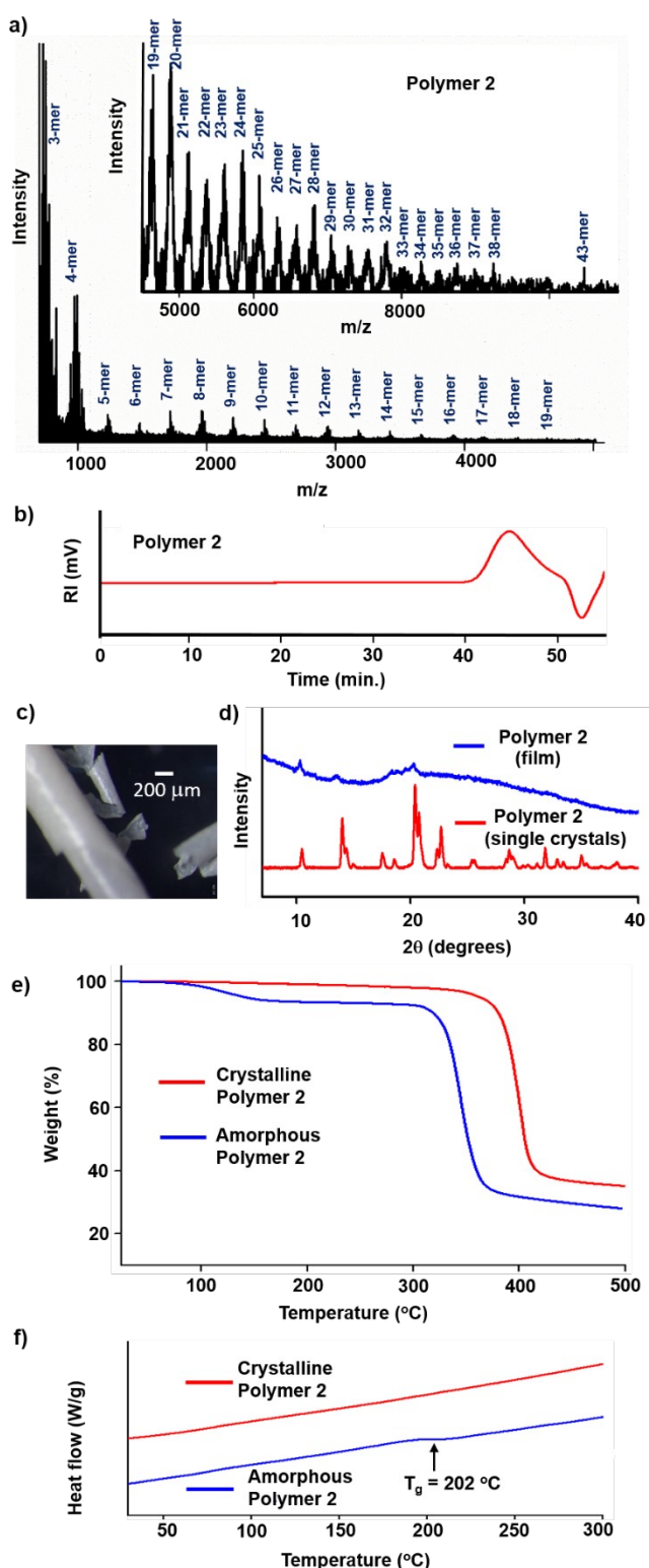
Fig. 6 a) MALDI spectrum and b) GPC elution curve for the polymer 2 . c) Photograph of the polymer 2 film. d) Comparison of PXRD patterns of polymer 2 single crystals and polymer 2 film. Comparison of e) TGA thermograms and f) DSC thermograms of crystalline and amorphous polymer 2 (heating rate: 5 °C/min.).
