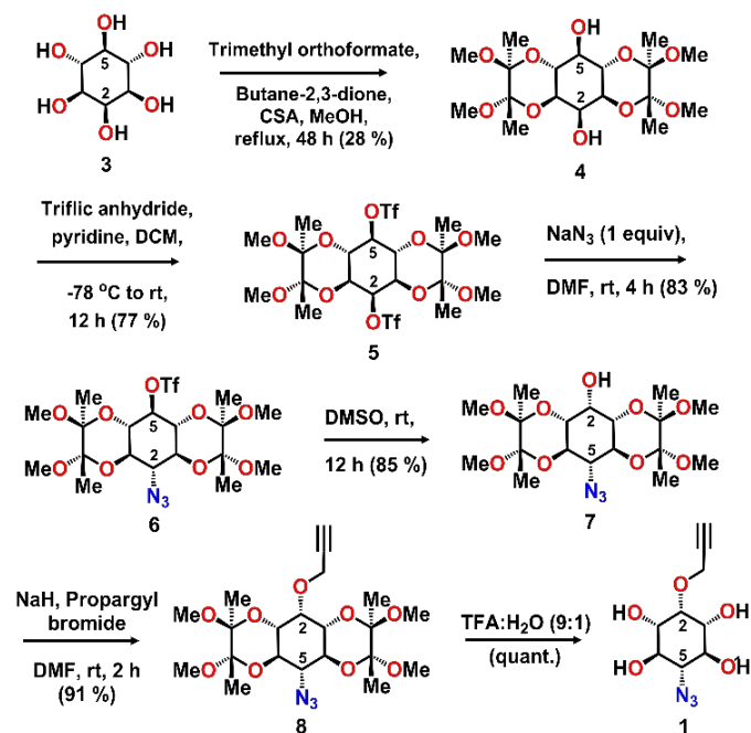
Scheme 1 Synthesis of tetrol 1 .
