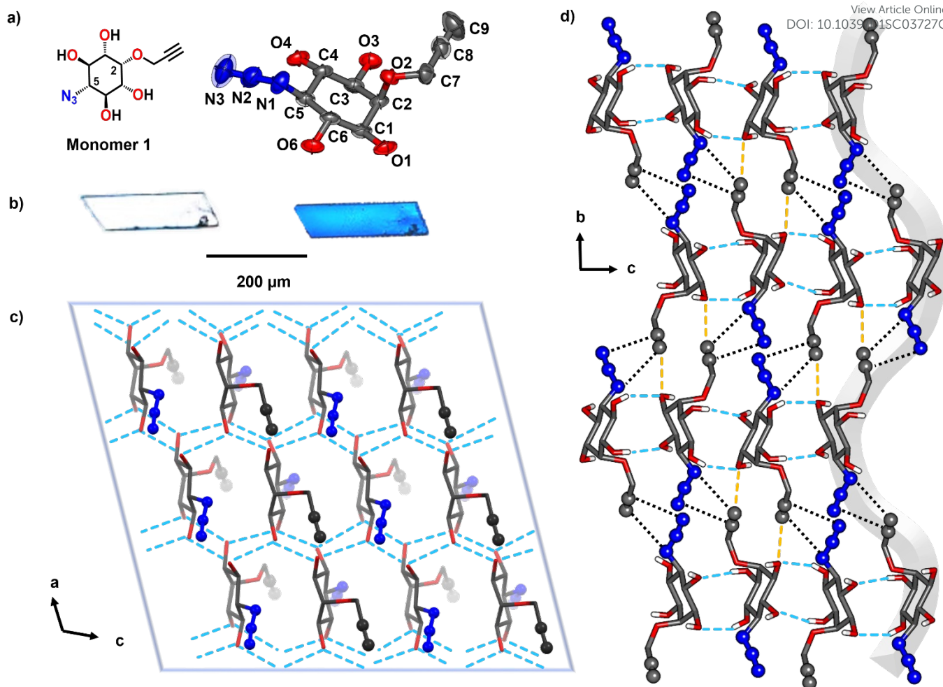
Fig. 3 a) Chemical structure and ORTEP diagram of tetrol 1 . The thermal ellipsoids are set at 50% probability. b) Photograph of the tetrol 1 single crystal taken under normal light and a polarizer. c) Crystal packing of the tetrol 1 in 'ac' plane showing a 2D hydrogen-bonded layer. d) Crystal packing viewed along 'a' direction. The OH...O hydrogen bonds and the CH...O hydrogen bonds are shown as blue and orange dotted lines, respectively. Black dotted lines represent the short contacts between the reactive terminals of antiparallely arranged azide and alkyne units. The direction of polymer chain growth is along the wavy line (along 'b' direction) shown in the background. H-atoms (except OH) are hidden for clarity.
