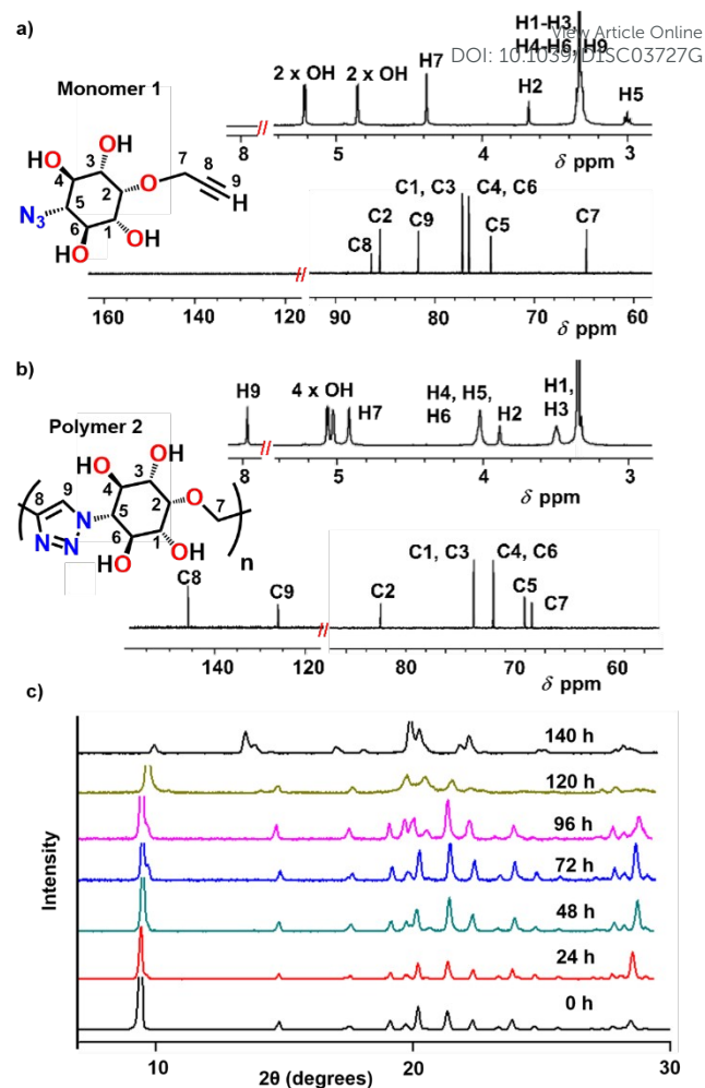
Fig. 4 ^1\text{H} NMR and ^{13}\text{C} NMR spectra of a) monomer 1 and b) polymer 2 recorded in \text{DMSO}-d_6 . c) Time-dependent PXRD analyses of monomer 1 heated at 80^\circ\text{C} .
