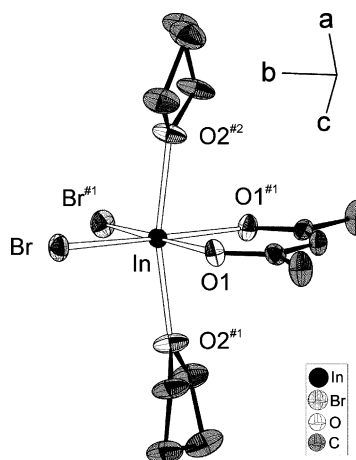
Fig. 3. Molecular structure of \text{In}(\text{acac})\text{Br}_2 \cdot 2\text{THF} .
