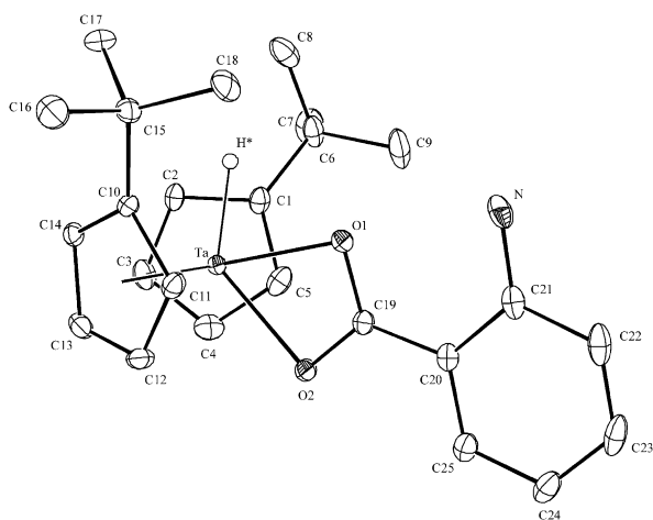
Fig. 1. ORTEP drawing of the cation [\text{Cp}_2'\text{Ta}(\text{H})(\text{aba})]^+ in 3 . Hydrogen atoms, except the hydride ( \text{H}^* ), are omitted for clarity. Selected bond distances (Å) and angles ( ^\circ ): Ta–CP1 2.082, Ta–CP2 2.070, Ta– \text{H}^* 1.65(4), Ta–O1 2.168(2), Ta–O2 2.177(2), CP1–Ta–CP2 132.7, O1–Ta–O2 59.47(7), O1–Ta– \text{H}^* 70(1), O2–Ta– \text{H}^* 129(1); CP1 and CP2 are the geometrical centers of C1–C5 and C10–C14 rings, respectively.
