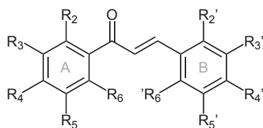
Fig. 1. Structure of the trans-chalcone, with the numbering used throughout the manuscript, and rings A and B highlighted in grey.
