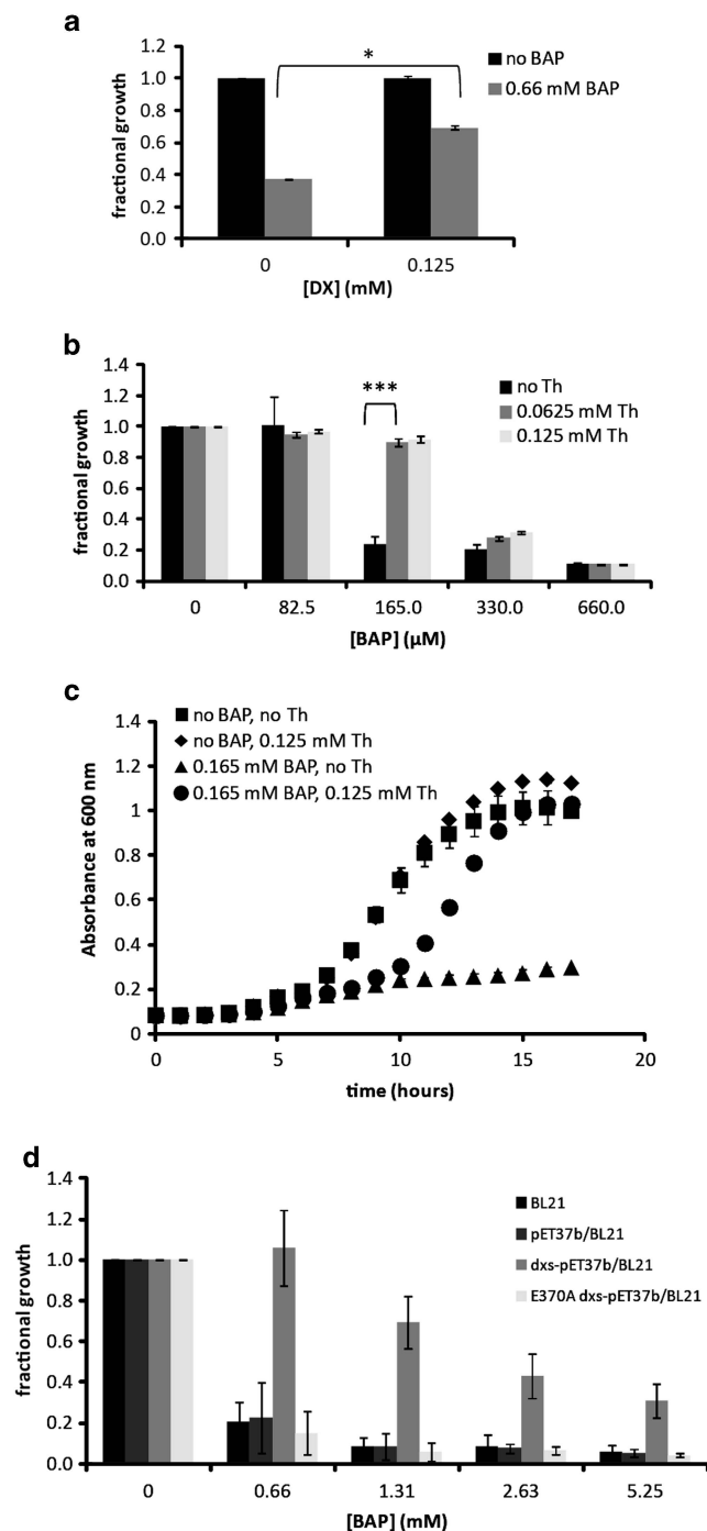
Figure 3 Butylacetylphosphonate (BAP) inhibition of E. coli MG1655 growth is rescued by 1-deoxy-D-xylulose (DX), thiamin (Th) and E. coli DXP synthase (Dxs) overexpression. (a) Fractional growth at 12.5h in the presence and absence of BAP and DX. Mean and standard error of four replicates are shown. *P = 0.022 (unpaired t -test comparing DX-treated and -untreated cultures at 0.66 mM BAP). (b) Fractional growth at 16h in the presence and absence of BAP and thiamin. Mean and standard error of four replicates is shown. ***P = 0.0000258 (unpaired t -test comparing thiamin-treated and -untreated cultures at 165 \mu\text{M} BAP). (c) Growth curve over 16h, in the absence or presence of BAP and thiamin. (d) Fractional growth at 16h determined for E. coli BL21 cells only, cells transformed with empty pET37b vector, vector-expressing recombinant E. coli DXP synthase protein ( dxs -pET37b) or vector expressing the catalytically inactive 15 E370A variant (E370A dxs -pET37b). Mean and standard error of four replicates is shown.
