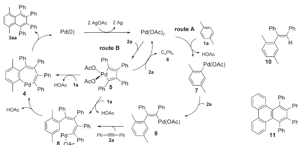
Scheme 1. Proposed mechanism for the formation of 3aa from alkyne 2a and p -xylene 1a .
