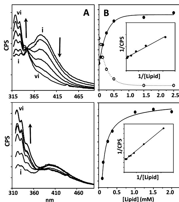
Figure 6. Fluorescence spectra at various lipid/compound ratios used to quantify partition equilibria. (Top) (A) Fluorescence emission spectra of 17 \mu M HO 2 C-Hex-Dip-Hex-C6 ( \lambda_{\text{max,ex}} = 305 nm) titrated against lipid vesicles. From line i to line vi , [lipid] = 0.0625, 0.125, 0.25, 0.5, 1.5, and 2.5 mM. (B) Counts per second (CPS) at 320 nm (black circles) and 380 nm (open circles) as a function of [lipid], double reciprocal plot (inset) used to determine K_p . (Bottom) Analogous data for HO 2 C-Hex-Dip-Hex-Hex-OH.
