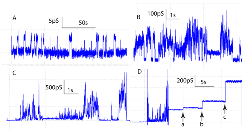
Figure 3. Conductance behaviors of compounds: (A) HO 2 C-Hex-Dip-Hex-Hex-OH, 1 M CsCl, +100 mV, 2 h after injection, (B) HO 2 C-Hex-Dip-Hex-Hex-OH, 1 M CsCl, +10 mV, 15 min after injection, same experiment as in (A), (C) HO 2 C-Hex-Dip-Hex-Hex-C6, 0.3 mol %, 1 M CsCl, +50 mV, (D) HO 2 C-Hex-Dip-Hex-Hex-OPhos, 0.3 mol %, 1 M CsCl, initially -175 to -150, -100, and -50 mV at points a–c.
