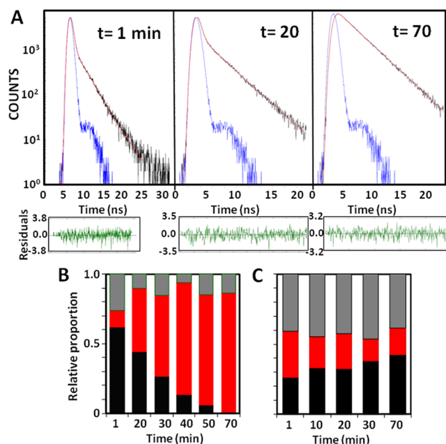
Figure 7. Time-resolved fluorescence lifetime measurements of compounds in vesicles: (A) TCSPC-derived fluorescence decay profiles monitored at 380 nm (276 nm excitation) for 20 \mu M HO 2 C-Hex-Dip-Hex-C6 incubated with a suspension of lipid vesicles in aqueous buffer (10 mM Na 3 PO 4 , 100 mM NaCl, pH 6.4) (blue, IRF; black, decay; red, fit to a triexponential), (B) change in relative proportions of each lifetime component over time for 20 \mu M HO 2 C-Hex-Dip-Hex-C6 (black, \tau_1 (shortest lived component); gray, \tau_2 (mid-lifetime component); red, \tau_3 (longest lived component), (C) analogous data for 20 \mu M HO 2 C-Hex-Dip-Hex-C12.
