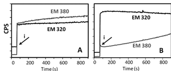
Figure 5. Emission spectra of compounds in the presence of vesicles. Fluorescence emission at 320 nm (black line) and 380 nm (gray line) over time of (A) 25 \mu M HO 2 C-Hex-Dip-Hex-C12 and (B) 25 \mu M HO 2 C-Hex-Dip-Hex-C6, injected at time i into an aqueous suspension of lipid vesicles (10 mM Na 3 PO 4 , 100 mM NaCl, pH 6.4).
