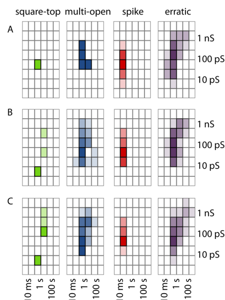
Figure 4. Summary activity grids of active compounds: (A) HO 2 C-Hex-Dip-Hex-Hex-C6, (B) HO 2 C-Hex-Dip-Hex-Hex-OH, (C) HO 2 C-Hex-Dip-Hex-Hex-OPhos.
