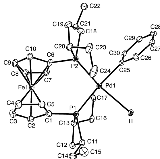
Figure 7. ORTEP diagram of one of the three independent molecules in the unit cell of Pd(( S,S )-Et-FerrolTANE)(Ph)(I)·0.33toluene ( 3g ·0.33(toluene)). The solvent molecule and disorder in one of the ethyl groups are not shown.
