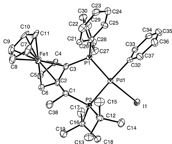
Figure 8. ORTEP diagram of Pd(( R,S )-PPF- t -Bu)(Ph)(I)·CH 2 Cl 2 ( 3i ·CH 2 Cl 2 ). Hydrogen atoms and the solvent molecule are omitted.
