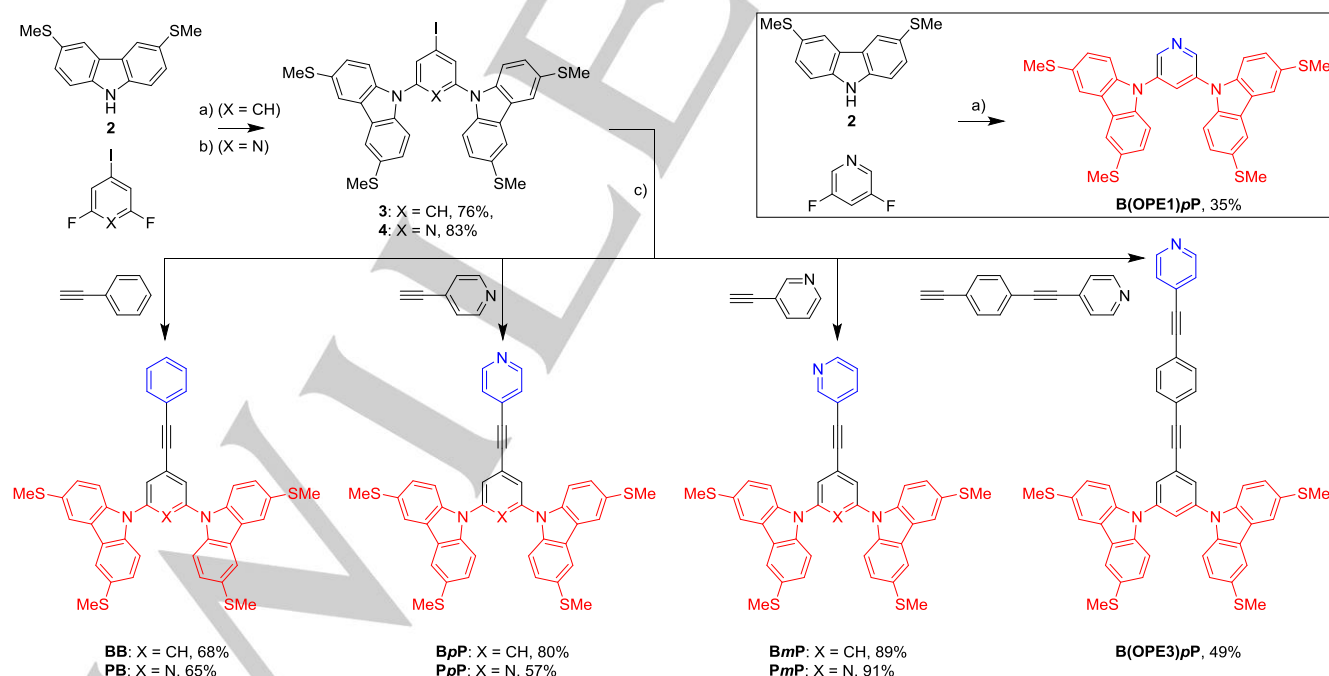
Scheme 1. Synthesis of tetrapodal molecular wires. Reagents and conditions: a) \text{Cs}_2\text{CO}_3 , DMF, 100 °C, 17 h; b) \text{K}_2\text{CO}_3 , DMSO, 70 °C, 2 h; c) \text{CuI} , \text{Pd}(\text{PPh}_3)_2\text{Cl}_2 , THF, DIPEA, RT, 80–120 min. For the tetrapodal molecular wires, the anchoring unit is coloured red, and the head unit blue (note that for B(OPE1)pP the head unit pyridine ring also forms part of the anchor group).
