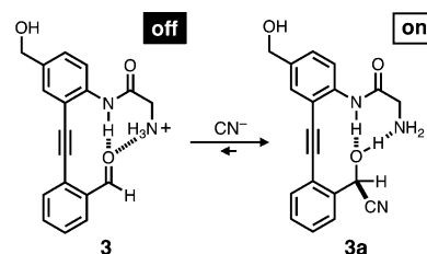
Scheme 5. Mechanism of Fluorescence Turn-On Detection of \text{CN}^- by Quencher-Modified Quantum Dot (Top) or by Quencher-Modified Fluorescent Dye Molecule, Such as 3 (Bottom)
