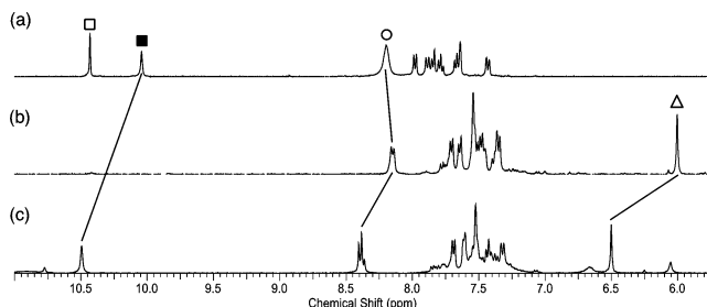
Figure 5. Partial ^1\text{H} NMR spectra of (a) 3 in \text{DMSO-}d_6 , (b) 3 + 5 equiv NaCN in \text{DMSO-}d_6/\text{D}_2\text{O} (5:2, v/v), and (c) 3 + 5 equiv (n\text{-Bu}_4\text{N})\text{CN} in \text{DMSO-}d_6 ; [\text{3}] = 4.5 \text{ mM} , T = 298 \text{ K} . The symbols \square , \blacksquare , \circ , and \Delta indicate the resonances of the aldehyde C–H, aniline amide N–H, ammonium N–H, and benzylic C–H proton, respectively. The lines indicate some corresponding signals. In (b), the amide N–H proton resonance disappears as a result of H/D exchange with \text{D}_2\text{O} .
