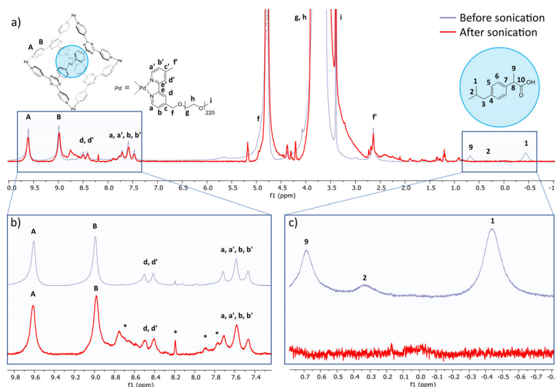
Figure 2. ^1\text{H} NMR ( \text{D}_2\text{O} , 298 K) of the encapsulated 1a ·(ibuprofen) 2 (blue line) and release of ibuprofen cargo (red line). Sonication time 3 h, a sequence of 1 s on and 1 s off was chosen, for each experiment only the “on” time is reported. The asterisks in the insets indicate the cage fragmentation products.
