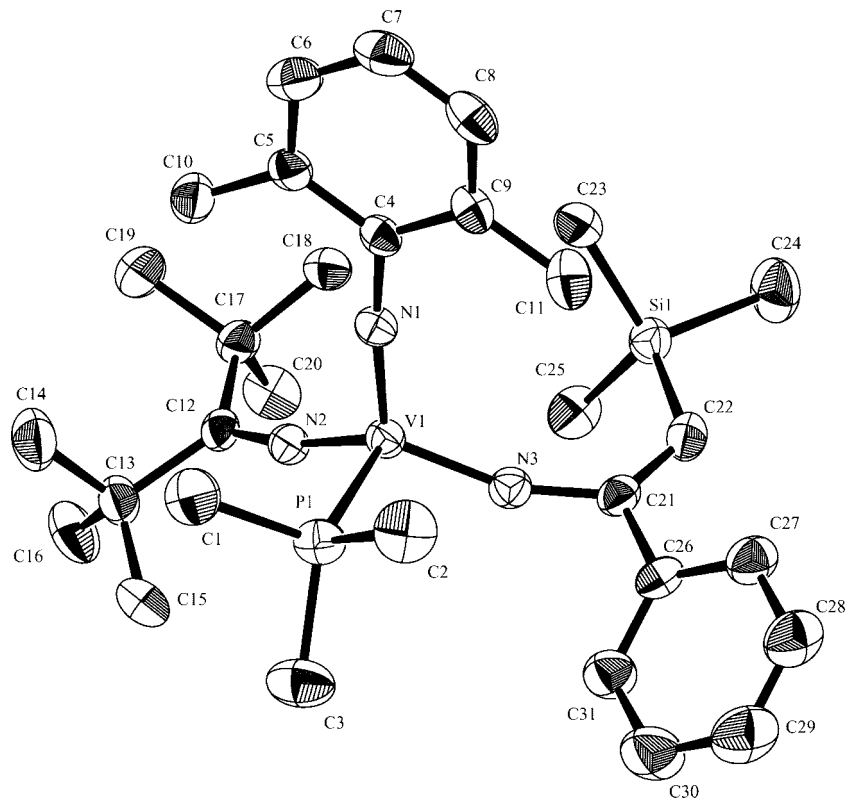
Figure 1. ORTEP drawings of \text{V}(\text{N}-2,6\text{-Me}_2\text{C}_6\text{H}_3)[\text{NC}(\text{Ph})=\text{CHSiMe}_3](\text{N}=\text{C}^t\text{Bu}_2)(\text{PMe}_3) ( 4 ). Thermal ellipsoids are drawn at the 50% probability level, and H atoms are omitted for clarity. 19
