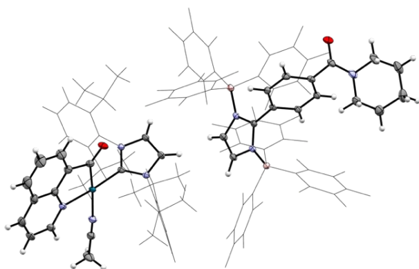
Fig. 5 Crystal structure of [1(MeCN)][IMP-pipA] . Ellipsoids shown at 50% probability; C 6 F 5 rings and diisopropylphenyl substituents shown in wireframe.
