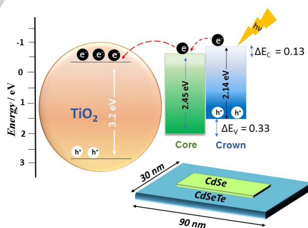
Figure 5. Electron energy diagram for core/crown CdSe/CdSeTe NPLs on TiO 2 .
