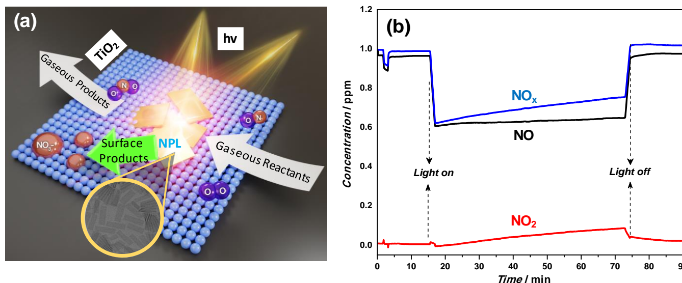
Figure 7. (a) Schematic representation of PHONOS process. (b) Concentration vs. time profiles for a typical PHONOS activity test performed with 0.1NPL/P25 under VIS irradiation. Red (bottom), black (middle) and blue (top) traces correspond to \text{NO}_2(\text{g}) , \text{NO}(\text{g}) and total \text{NO}_x (i.e. \text{NO}(\text{g}) + \text{NO}_2(\text{g}) ) concentrations, respectively. Feed composition: \text{N}_2(\text{g}) 0.750 SLM, \text{O}_2(\text{g}) 0.250 SLM, and \text{NO}(\text{g}) 0.010 SLM (100 ppm \text{NO}(\text{g}) diluted in balance \text{N}_2(\text{g}) , 50% relative humidity (RH) at 23 °C.
