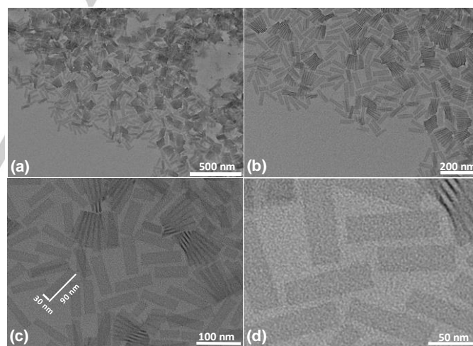
Figure 2. (a-d) Representative TEM images of CdSe/CdSeTe NPLs with different magnifications.
