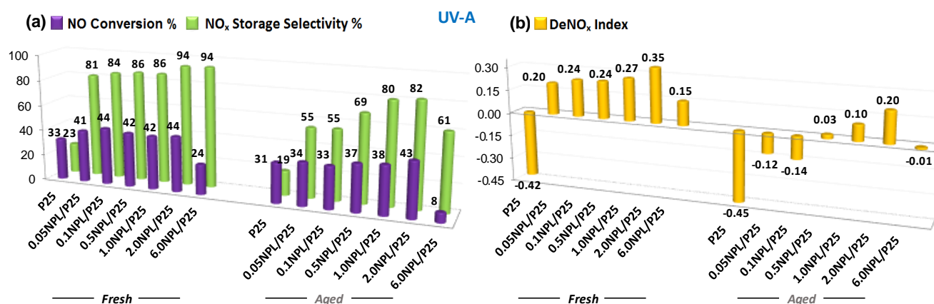
Figure 8. NO(g) conversion %, NO x storage selectivity % and DeNO x index values for different NPL/P25 composite photocatalysts obtained under UV-A irradiation.
