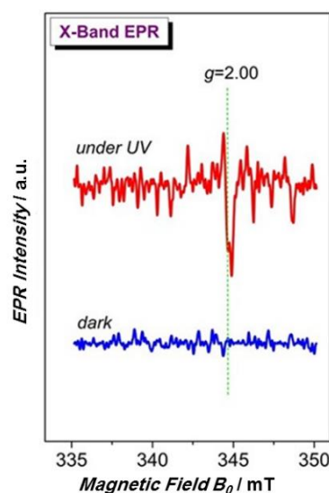
Figure 6. Room temperature X-band EPR spectra of CdSe/CdSeTe NPLs (without TiO 2 ) under dark and UV illumination conditions.
