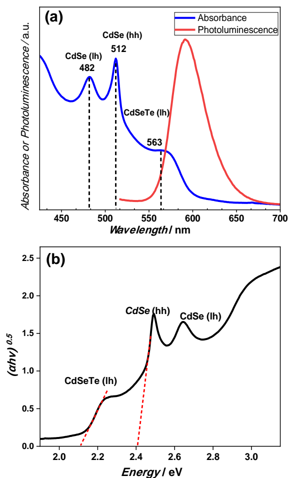
Figure 4. (a) Absorbance and photoluminescence spectra of 4 ML-thick bare CdSe/CdSeTe NPLs ( i.e. without TiO 2 ) dispersed in toluene; (b) Tauc plot for bare CdSe/CdSeTe NPLs.
