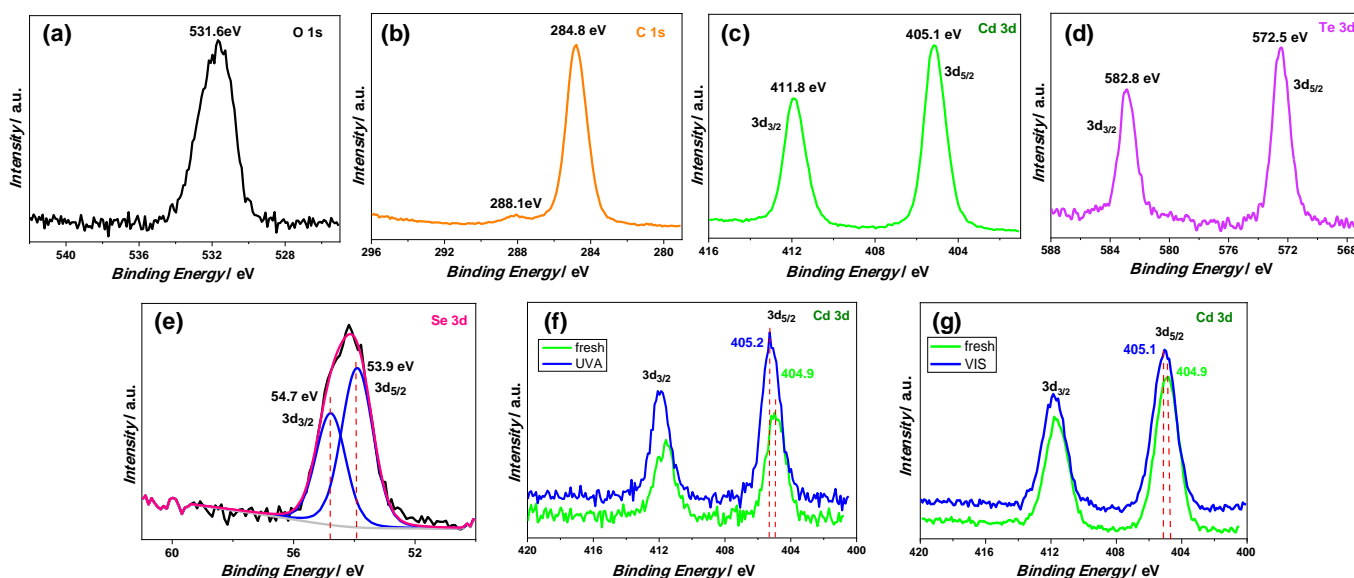
Figure 3. XPS spectra of fresh (as prepared) CdSe/CdSeTe NPLs (in the absence of TiO 2 ): (a) O 1s, (b) C 1s, (c) Cd3d, (d) Te3d, and (e) Se3d regions. Cd3d XPS spectra for CdSe/CdSeTe/TiO 2 (P25) composites before (green) and after (blue) 5 h PHONOS reaction under (f) UV-A, and (g) VIS illumination.
