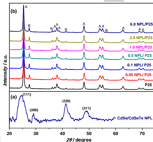
Figure 1. XRD patterns of (a) CdSe/CdSeTe NPLs (without TiO 2 ), and (b) pure P25, and CdSe/CdSeTe/P25 composite materials with various NPL loadings. A: anatase, R: rutile.
