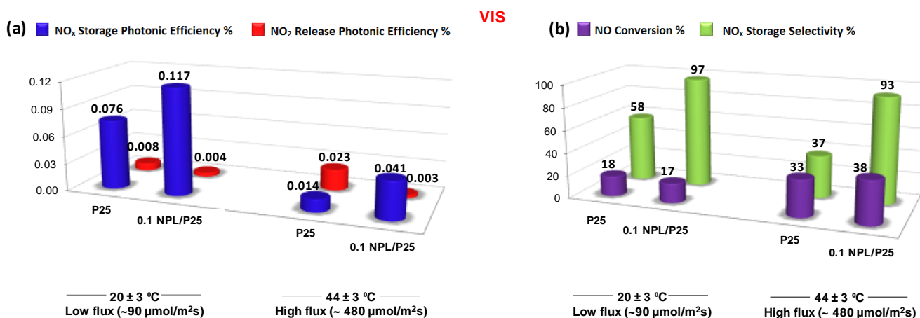
Figure 12. Temperature-dependent PHONOS data for pure P25 and 0.1NPL/P25 under VIS-light illumination (a) \text{NO}_x storage photonic efficiency % and \text{NO}_2 release photonic efficiency %, (b) NO conversion % and \text{NO}_x storage selectivity % values.
